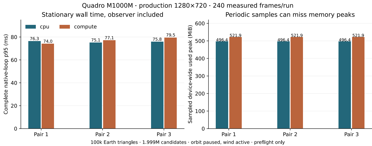
Figure 7: Production native stationary preflight, three alternating pairs. Complete loop p95 includes the private observer; physical memory shows periodic device-wide sampled maxima and can miss true peaks. All six runs retain matching scalar workloads. These are neither replacement-memory gates nor an accepted migration speedup.
