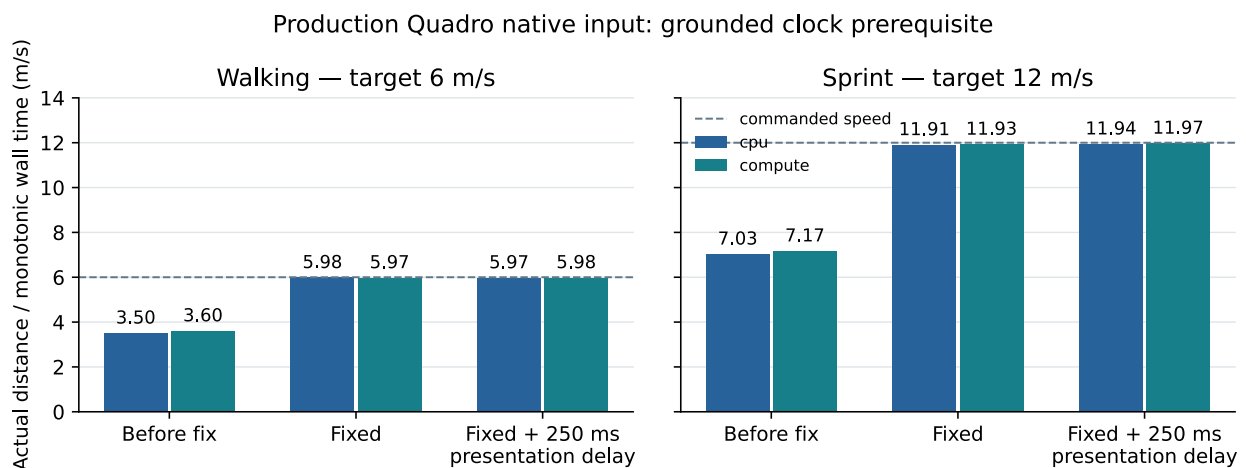
Figure 8: Actual grounded distance per monotonic wall second on production Quadro native input. Baseline uses short routes; fixed natural and delayed checks use 100 m. Each bar is one input run, with full raw spikes retained; these are speed prerequisites, not paired route cost acceptance or uncertainty estimates.
