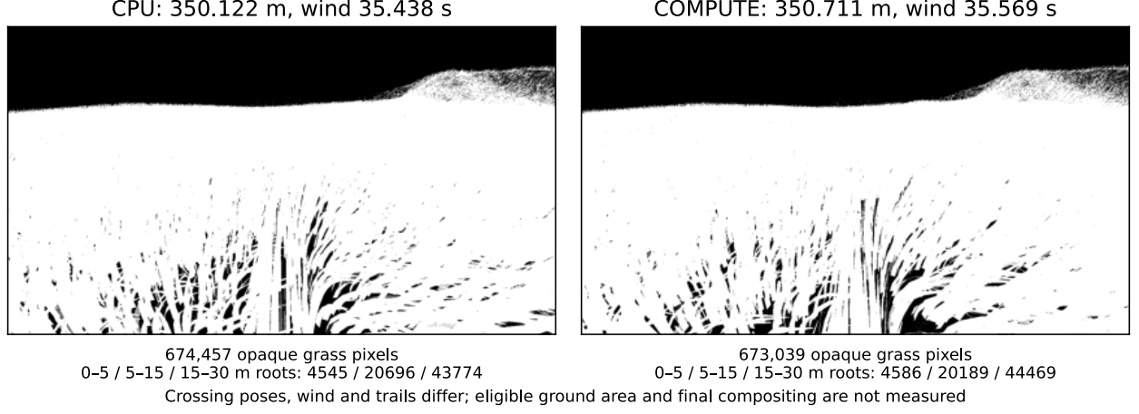
Figure 10: Illustrative actual native grass depth-change masks on production Quadro sprint. White pixels mark nearest opaque fragments changed by grass. Crossing pose, wind and trail states differ. Eligible visible ground area and final compositing are not measured, so these observations do not establish rendered density parity.
