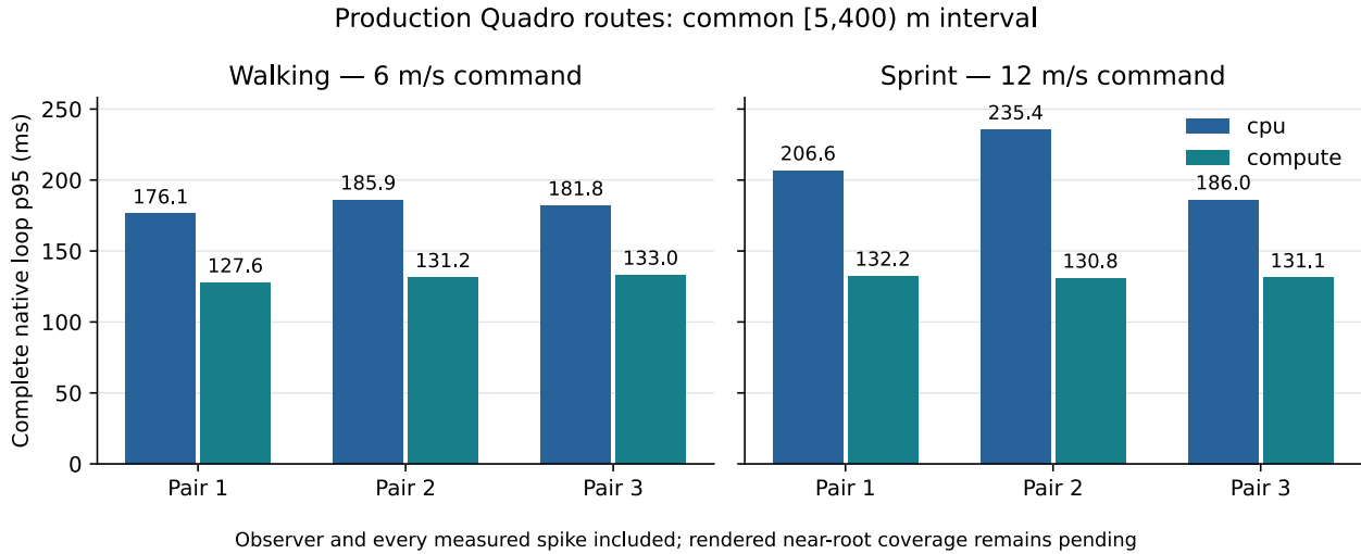
Figure 9: Complete native route p95 on production Quadro. Each pair covers the common interval from 5 m to less than 400 m at commanded walking/sprint speed. Observer overhead and every measured spike remain included. Rendered near-root coverage is pending; these bars do not establish accepted migration speedups or uncertainty bounds.
