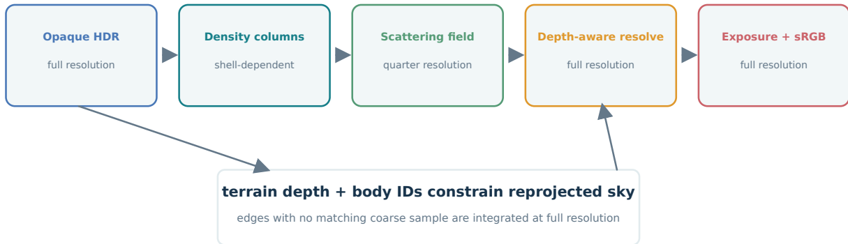
Figure 19: Atmospheric rendering graph. A reusable density-column lookup and a reduced scattering field lower repeated work; full-resolution depth controls edge reconstruction. Generated schematic.
