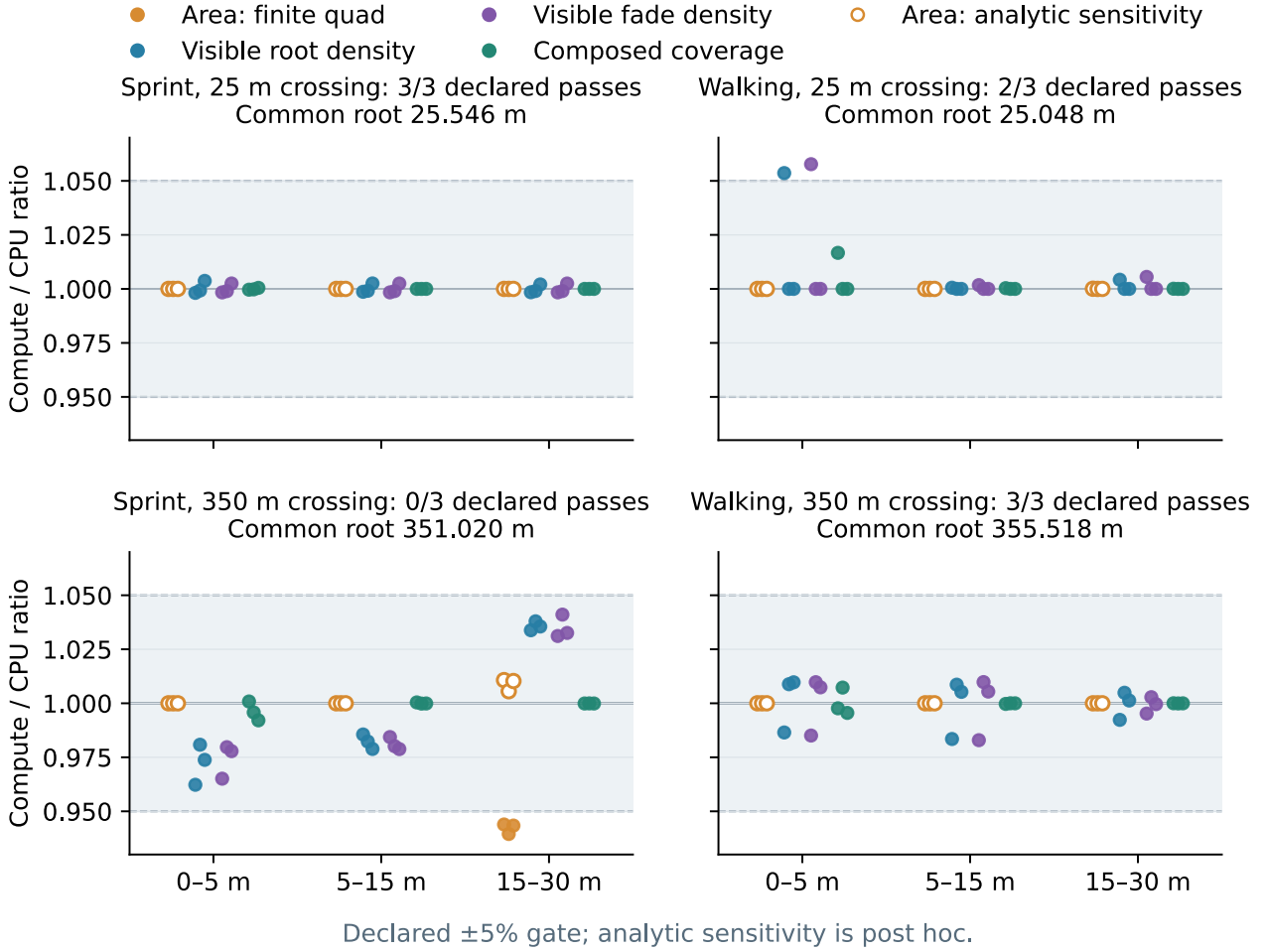
Figure 11: Declared common-view coverage ratios on three alternating pairs per crossing/case. Filled markers use the original finite-quad area proxy; open orange markers are post hoc analytic area sensitivity. Shading marks \pm 5\% . Eight of twelve primary pairs pass; no corrected-method or migration acceptance is claimed. Actual common root distances appear in each panel.
