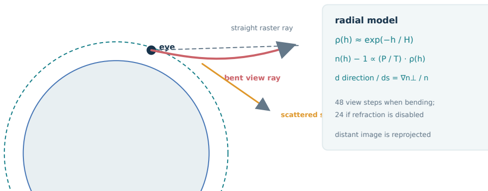
Figure 16: A refractive view ray bends through denser air while solar light contributes scattered radiance. Near terrain keeps its rasterized silhouette; only visible distant imagery is reprojected. Generated schematic.
