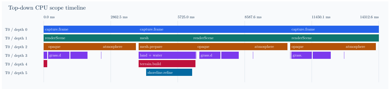
Figure 26: Top-down nested CPU scope timeline for three frozen walking frames on llvmpipe. Width represents wall time, including waits.
