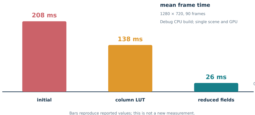
Figure 20: Reported mean frame times from README.md, Quadro M1000M, 1280 \times 720 , 90 frames. These bars visualize previously reported measurements, not a new benchmark.
