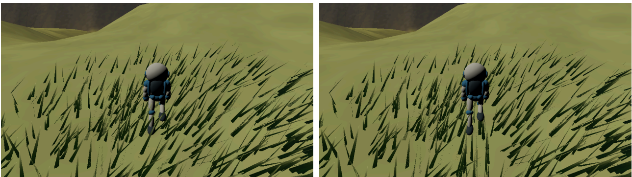
Figure 37: Identical pose, terrain, foliage roots and wind phase: unpressed control (left), persistent walking trail (right). The six-metre walk records 20 segments with 977 GPU-submitted blades; its replay is byte-identical.
