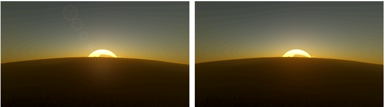
Figure 27: Production-start dense offline view: stronger, spread aperture ghosts and solar streak (left), identical scene with flare disabled (right). The dense PNG replays byte-identically. These are direct native-resolution renderer captures.
