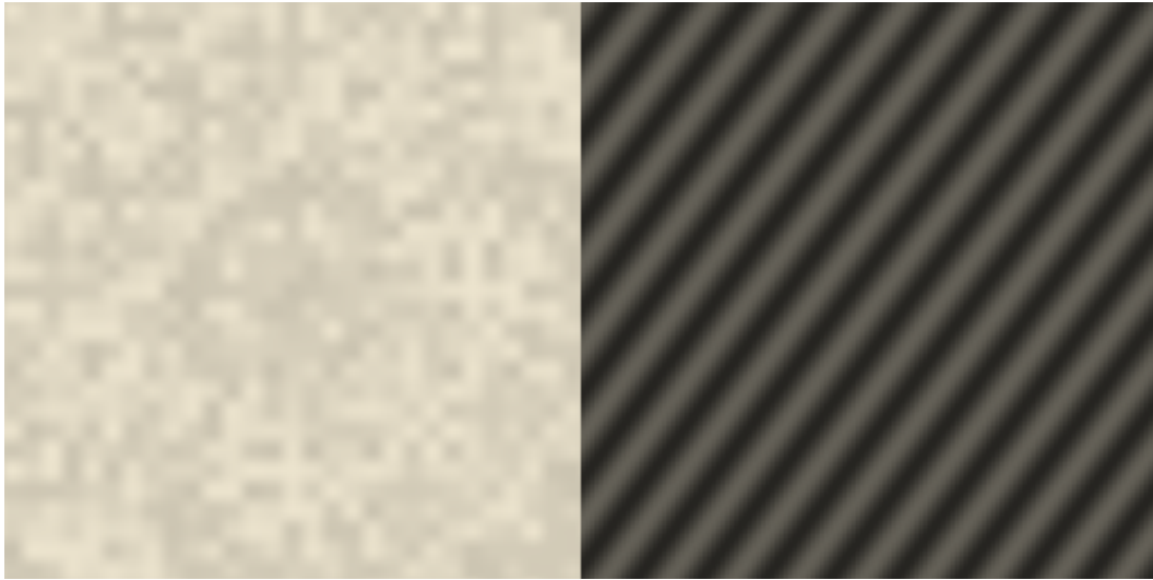
Figure 24: Production-shader diagnostic: fine grain across a 16 cm patch under indirect light (left), and wind ripples across a 2 m patch under grazing sunlight (right). Two triangles per patch, with unchanged depth; scales and lighting differ deliberately.
