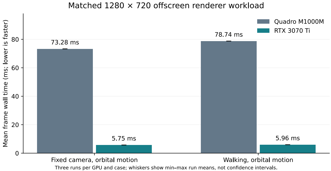
Figure 23: New matched physical-GPU measurements. Bars average three run means; whiskers show observed min-max run means, not confidence intervals. This uncapped offscreen comparison does not measure desktop presentation or native interactive FPS.
