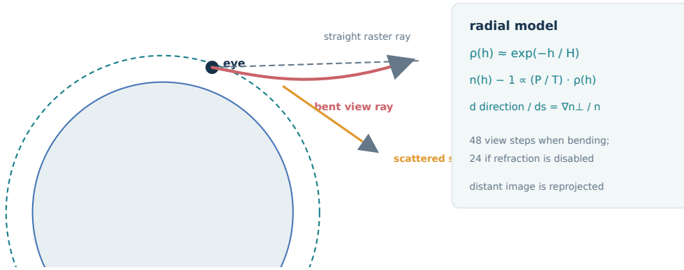
Figure 18: A refractive view ray bends through denser air while solar light contributes scattered radiance. Near terrain keeps its rasterized silhouette; only visible distant imagery is reprojected. Generated schematic.
