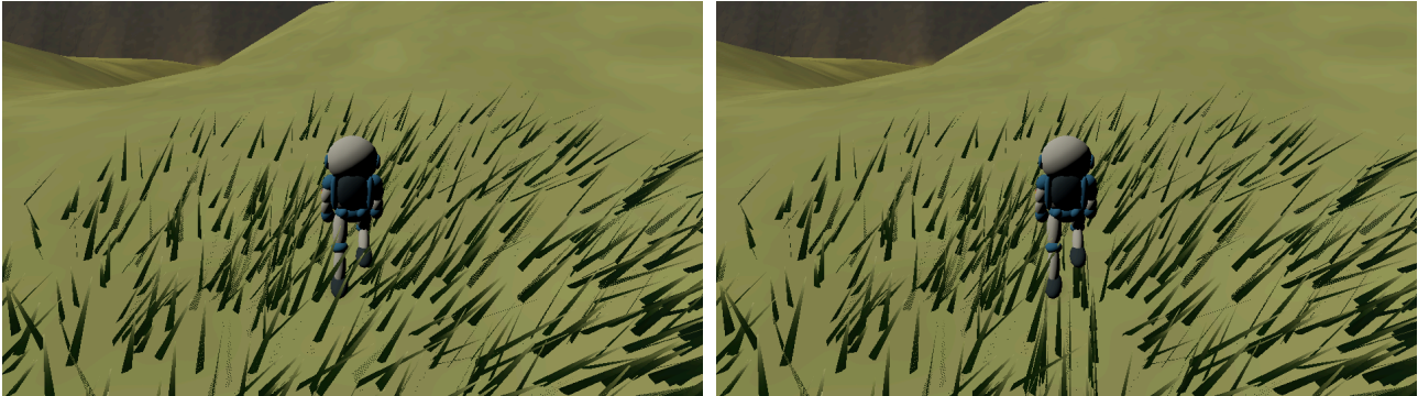
Figure 39: Identical pose, terrain, foliage roots and wind phase: unpressed control (left), persistent walking trail (right). The six-metre walk records 20 segments with 977 GPU-submitted blades; its replay is byte-identical.
