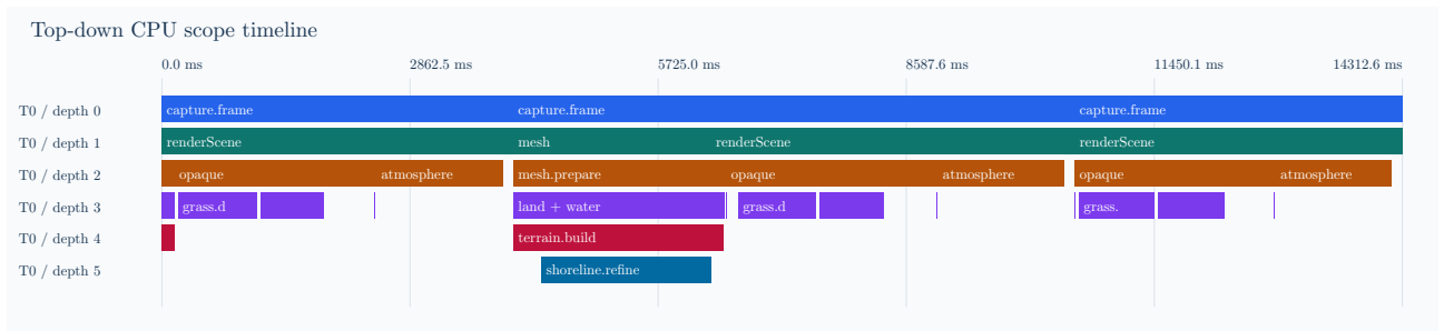
Figure 28: Top-down nested CPU scope timeline for three frozen walking frames on llvmpipe. Width represents wall time, including waits.
