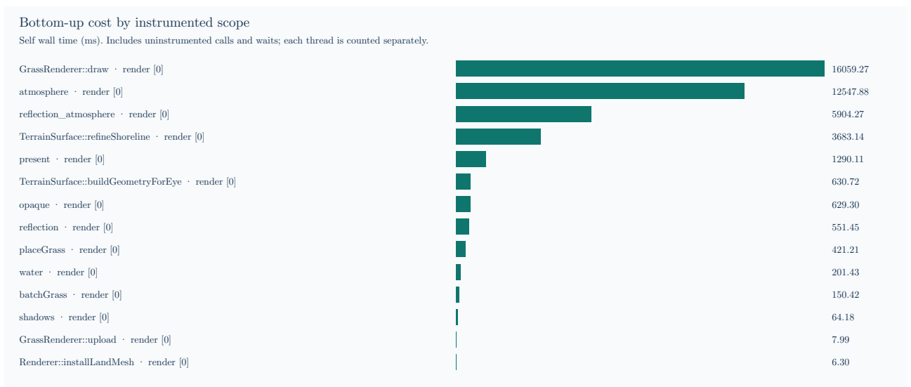
Figure 29: Bottom-up self wall time over ten walking frames. Immediate child scopes are subtracted; uninstrumented work and waits remain.
