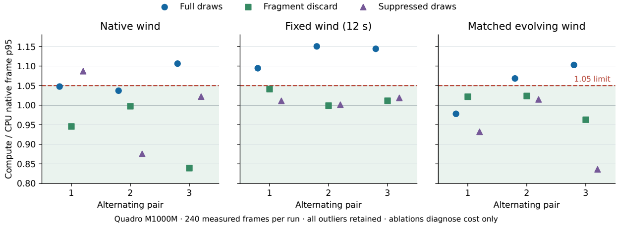
Figure 13: All 27 stationary Quadro pair ratios. Full draws execute the production grass path; discard retains placement/vertex work but disables rasterization; suppression omits grass draws after placement. The dashed 1.05 limit applies to full-draw costs. Ablations diagnose work and cannot qualify migration. All outliers remain.
