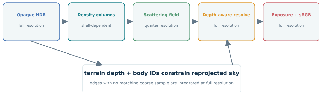
Figure 21: Atmospheric rendering graph. A reusable density-column lookup and a reduced scattering field lower repeated work; full-resolution depth controls edge reconstruction. Generated schematic.
