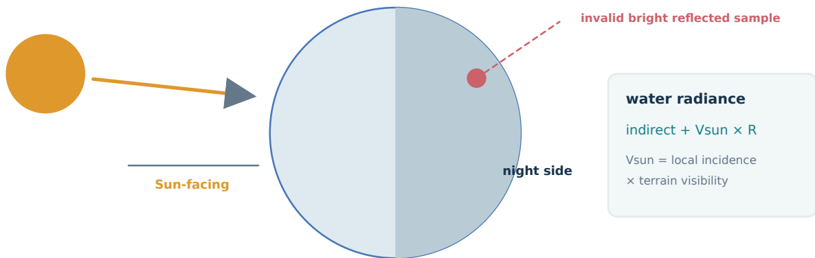
Figure 32: A reflected bright sample can exist in image space even when the water point lies on the night side. Local incidence and shadow-map visibility gate the direct reflection term. Generated schematic.
