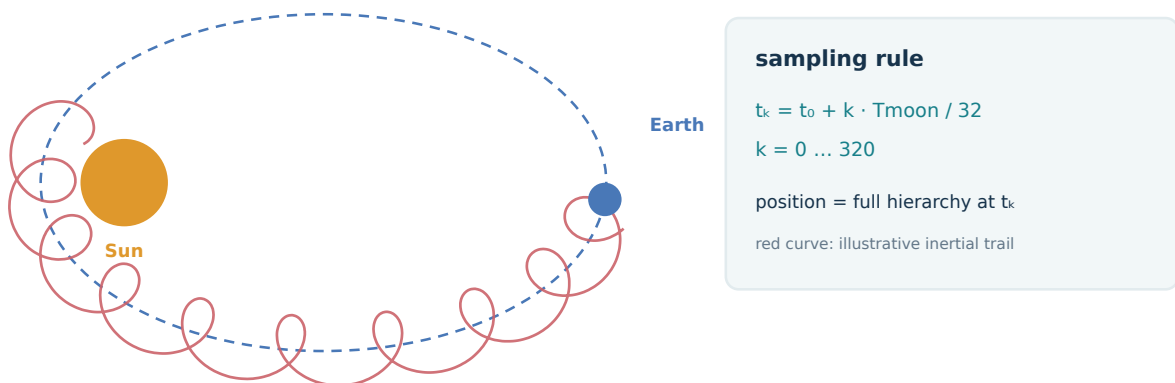
Figure 15: Illustrative moon trail in the inertial world frame. The repeated local cycles travel with the parent; the curve is explanatory and does not plot a measured scenario trajectory. Generated schematic.
