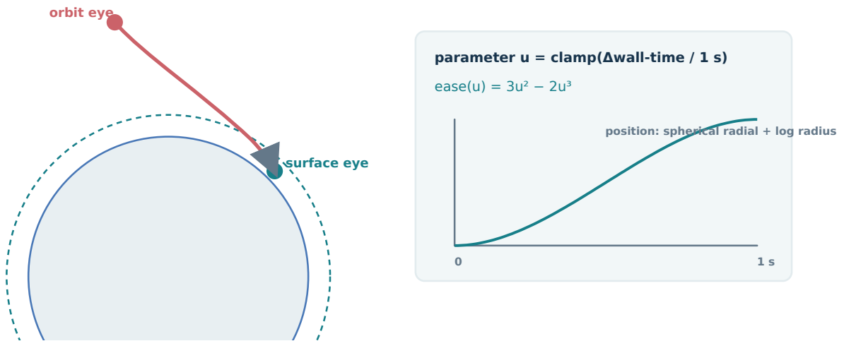
Figure 34: Orbit-to-surface descent. The curve shows the implemented smoothstep parameter; the spatial path is schematic because the actual start, target, and terrain vary by scene.
