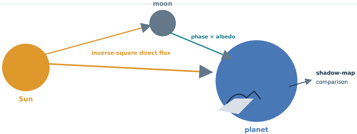
Figure 16: The Sun contributes direct flux to each body, the Moon reflects a phase-dependent portion toward the planet, and terrain visibility controls direct light. The diagram is schematic; arrow widths do not encode flux.
