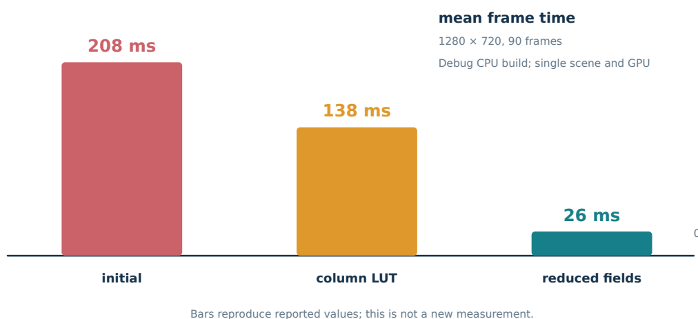
Figure 22: Reported mean frame times from README.md, Quadro M1000M, 1280×720, 90 frames. These bars visualize previously reported measurements, not a new benchmark.
