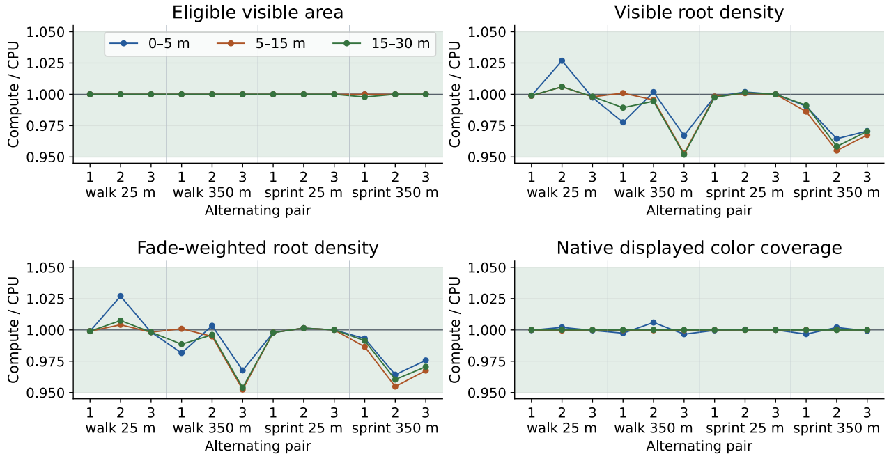
Figure 12: Fresh qualified Quadro comparisons: three alternating pairs for each nominal crossing/case, with native generations retained. All bands meet the shaded \pm 5\% gate. Color measures a native display-grid proxy with separately recorded edge-area uncertainty, not physical supersampled blade coverage. Every route frame is excluded from timing acceptance.
