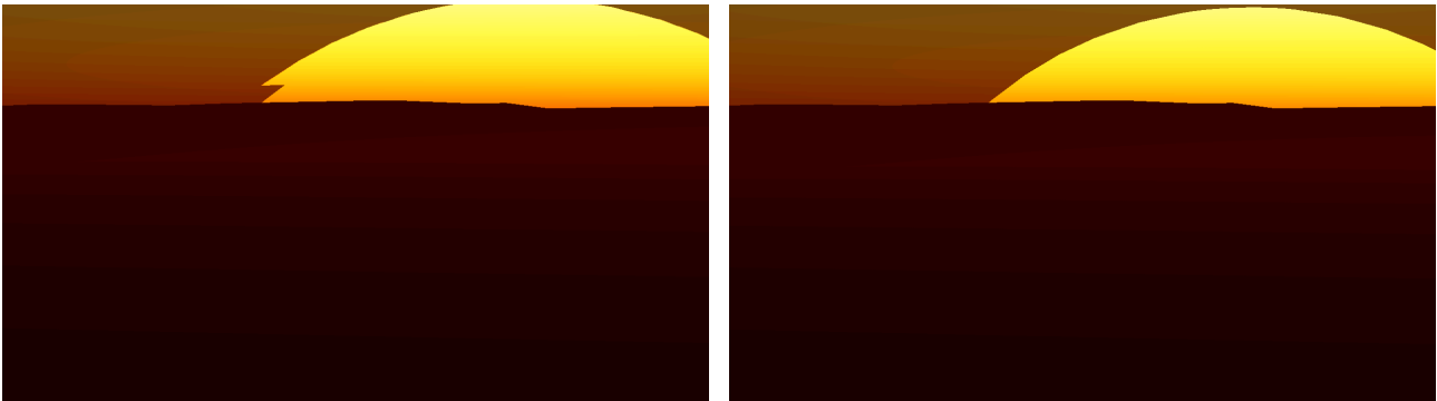
Figure 16: Matched full-resolution renderer captures of extreme refraction enabled (left) and disabled (right). Only the JSON bending switch changes; scattering and exposure remain active in both.
