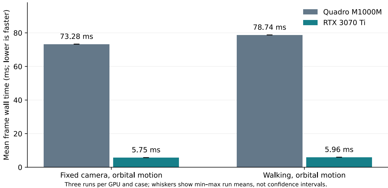
Figure 20: New matched physical-GPU measurements. Bars average three run means; whiskers show observed min-max run means, not confidence intervals. This uncapped offscreen comparison does not measure desktop presentation or native interactive FPS.
