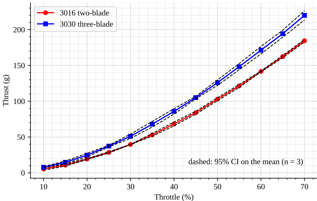
FirstName LastName's Thrust Curve Plot 2026-11-10
