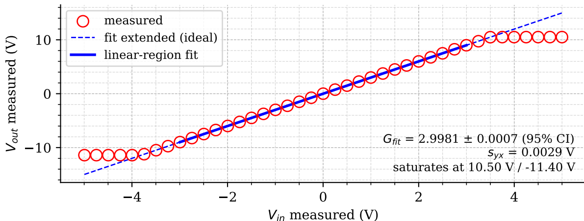
LM358 non-inverting amplifier — expected G = 2.9970
