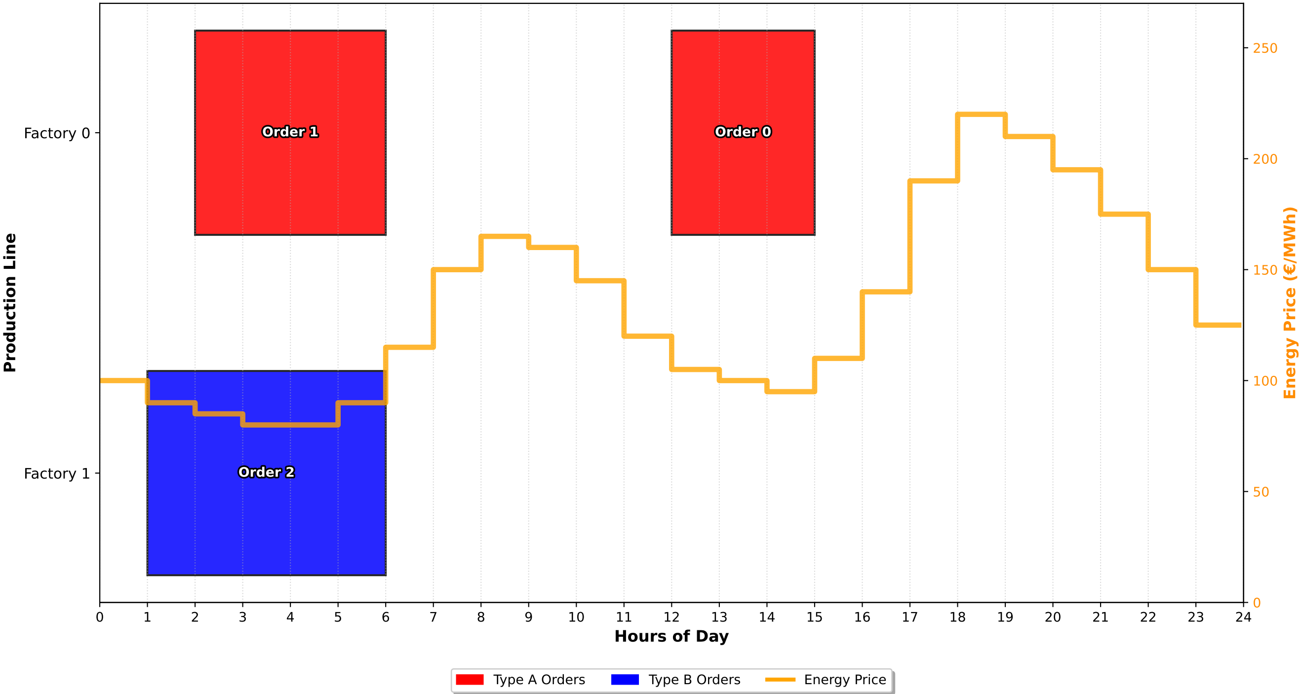
Combined Schedule & Energy Cost Profile
