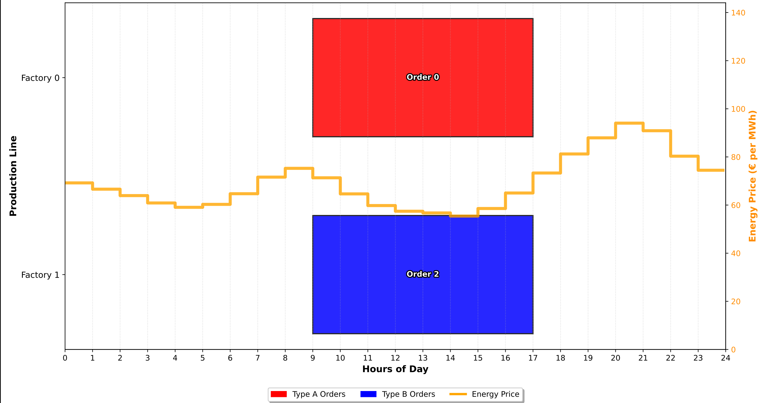
Combined Schedule & Energy Cost Profile - Scenario 0 (p=0.8677)
