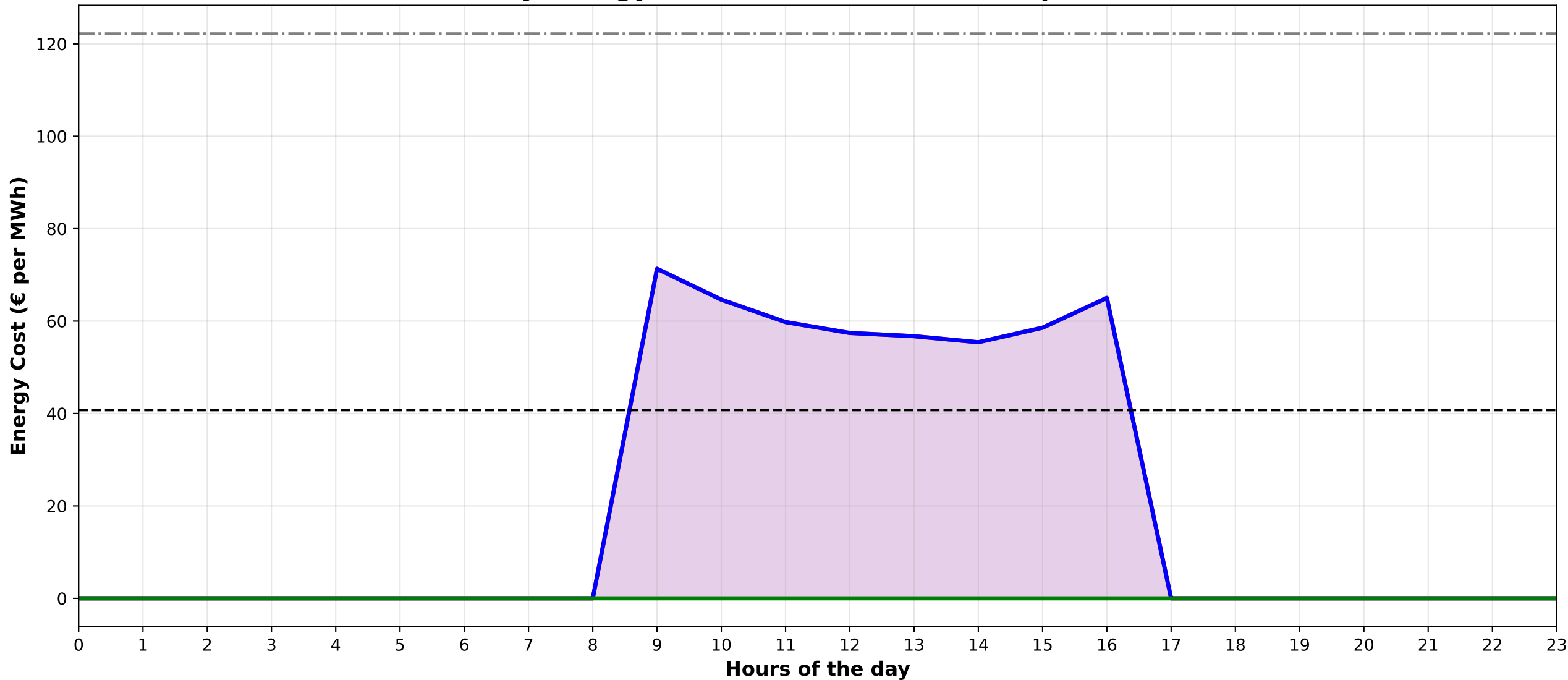
Hourly Energy Cost Profile - Scenario 0 (p=0.8677)
