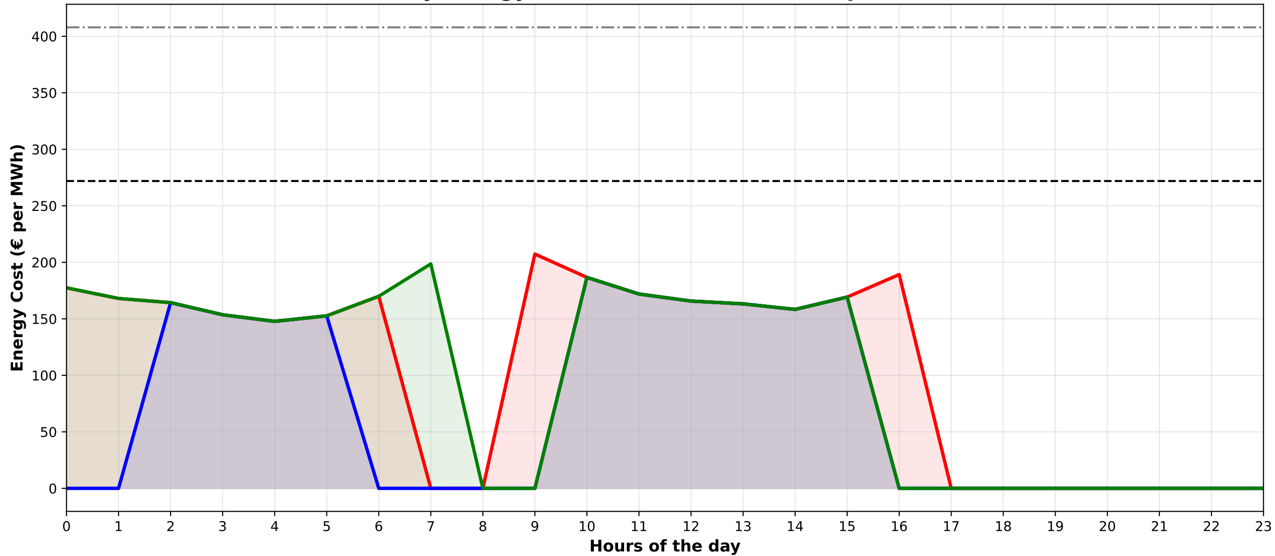
Hourly Energy Cost Profile - Scenario 1 (p=0.1489)
