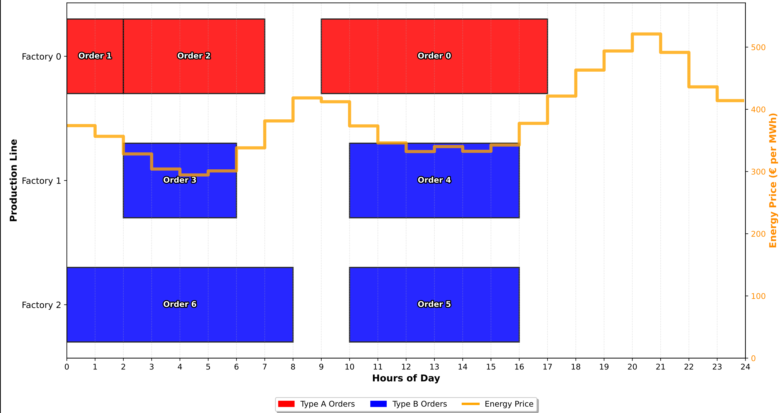
Combined Schedule & Energy Cost Profile - Scenario 2 (p=0.0326)
