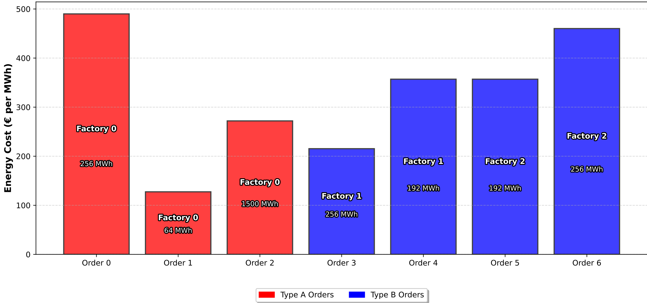
Energy Cost per Order - Scenario 0 (p=0.8185) - Colored by Type
