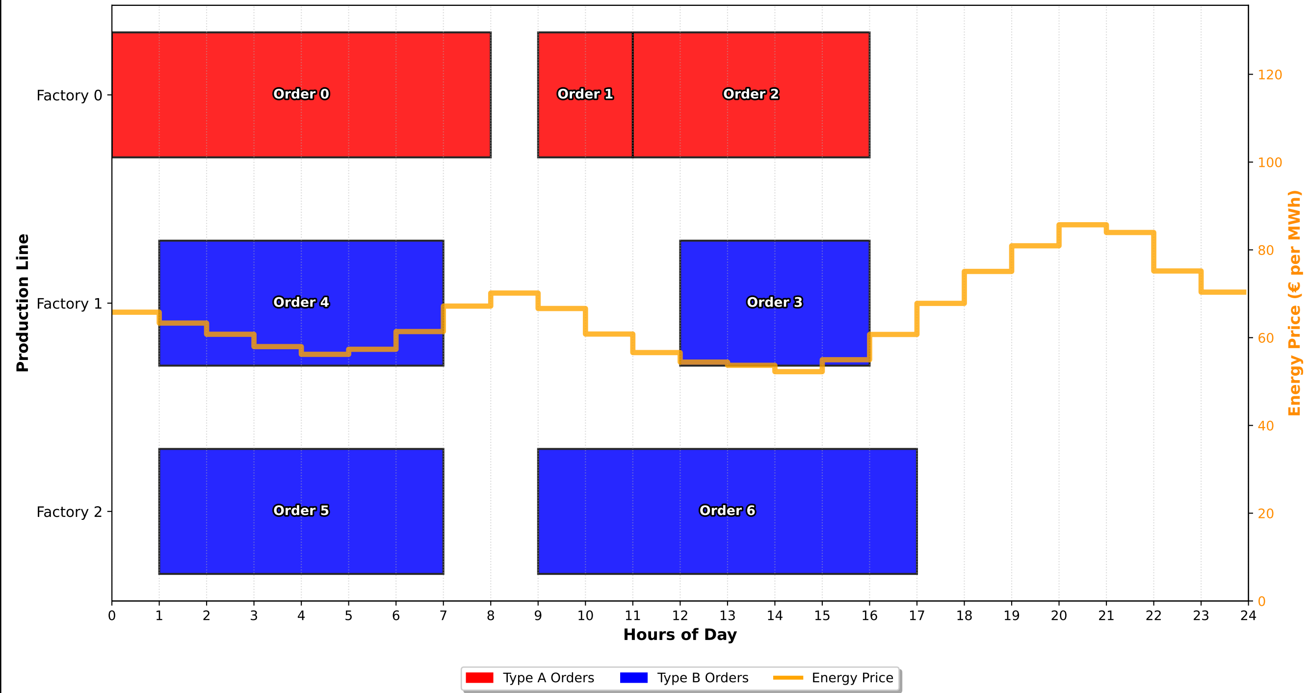
Combined Schedule & Energy Cost Profile - Scenario 0 (p=0.8185)
