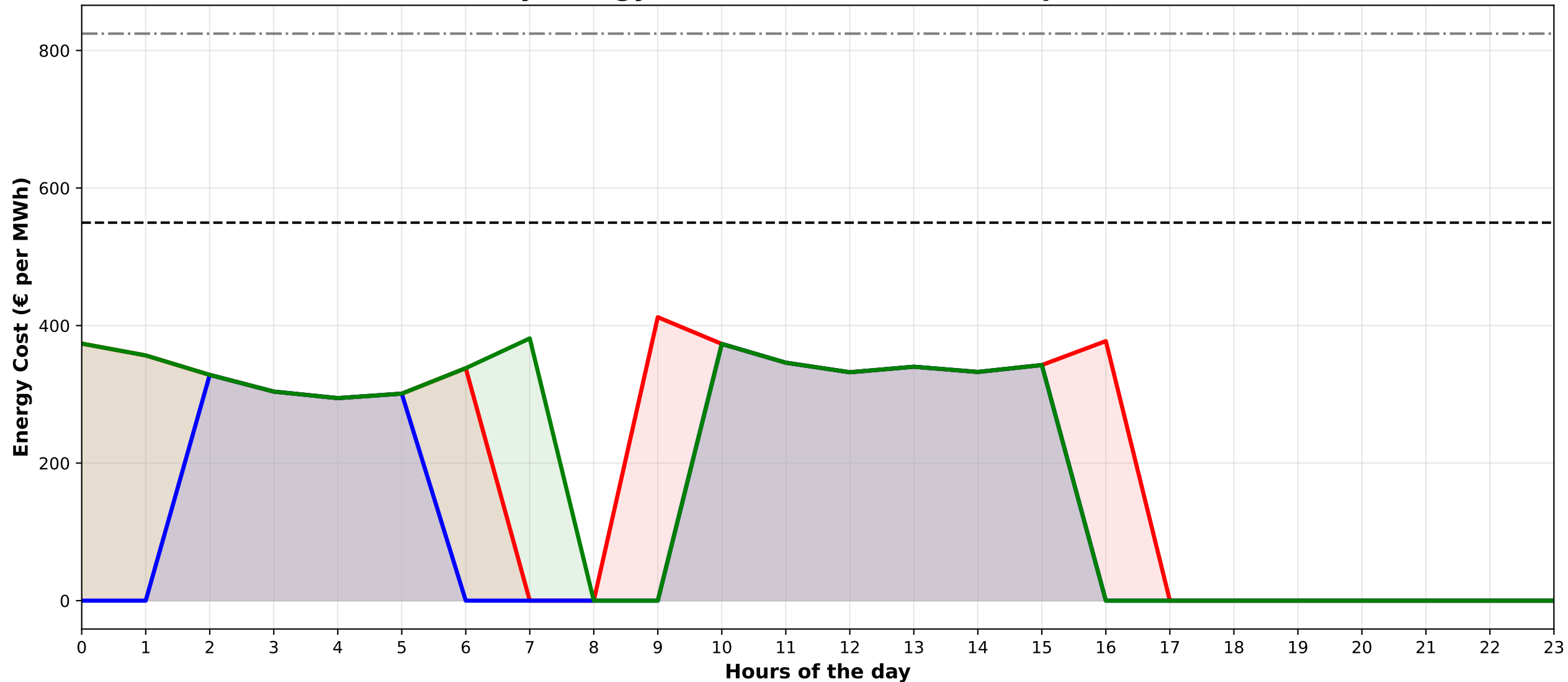
Hourly Energy Cost Profile - Scenario 2 (p=0.0326)
