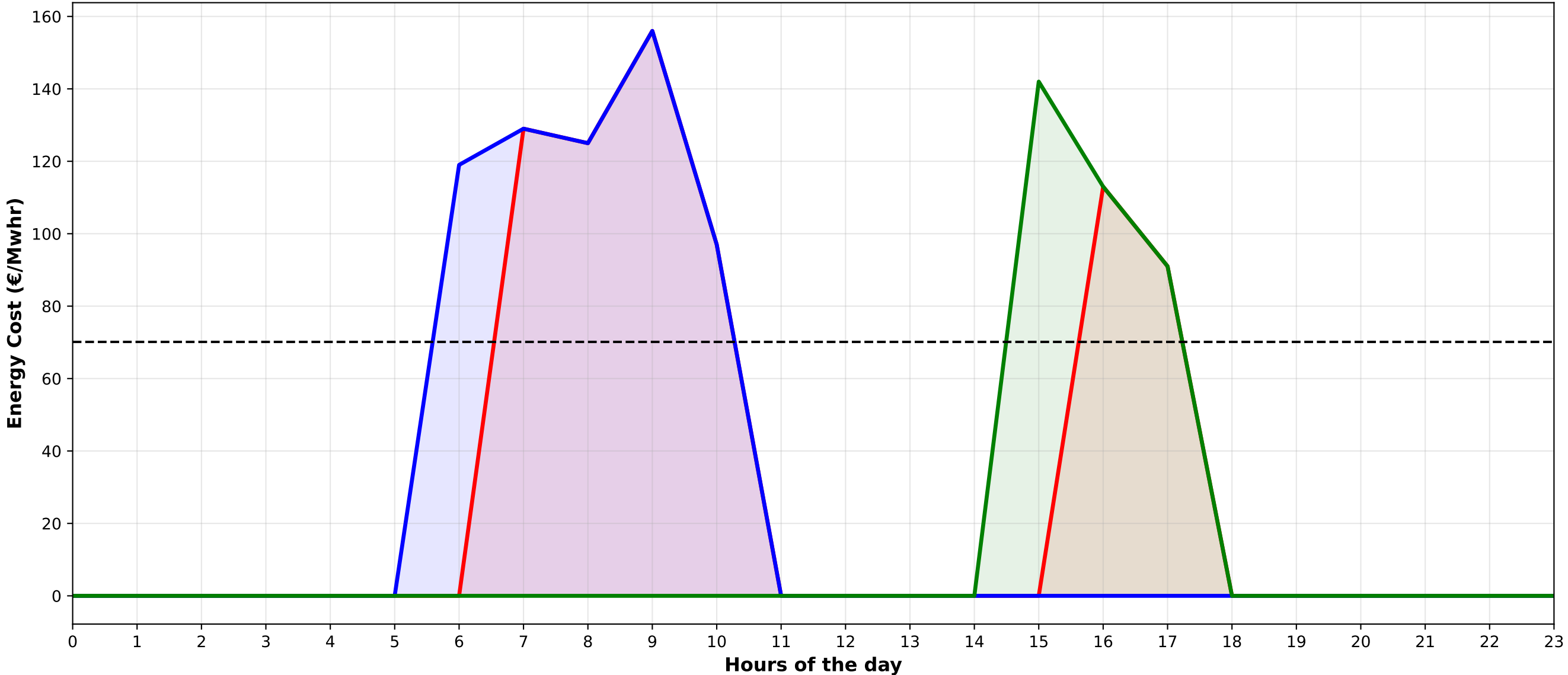
Hourly Energy Cost Profile per Factory Type
