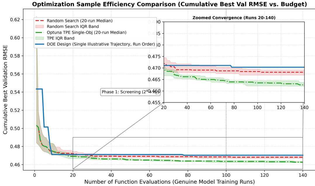
Figure 5: Sample Efficiency Convergence: Cumulative best validation RMSE vs. evaluation budget. Curves for Random Search and TPE show median trajectories \pm IQR shaded bands across 20 independent runs. The sequential DOE curve shows cumulative best in actual randomized run execution order. Inset highlights fine-grained convergence between runs 20 and 140.
