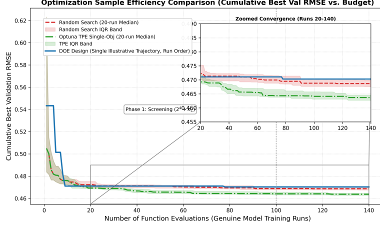
Figure 6: Sample Efficiency Convergence: Cumulative best validation RMSE vs. evaluation budget. Curves for Random Search and TPE show median trajectories \pm IQR shaded bands across 20 independent runs. The DOE curve shows cumulative best in actual randomized run execution order across the pre-planned blocked design. Inset highlights fine-grained convergence between runs 20 and 140.
