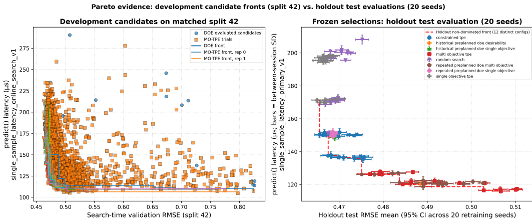
Figure 5: Pareto Evidence Architecture: (Left) Development candidate Pareto fronts on matched split 42 under the online 30-call latency protocol, showing evaluated DOE points, MO-TPE search trial clouds, and replicate-level candidate Pareto steps; (Right) Evaluated frozen selections on the external holdout test set across 20 retraining seeds, with horizontal error bars showing 95% confidence intervals for holdout test RMSE and vertical error bars showing between-session latency standard deviations. The red dashed line traces the empirical holdout non-dominated front comprising 12 distinct configurations.
