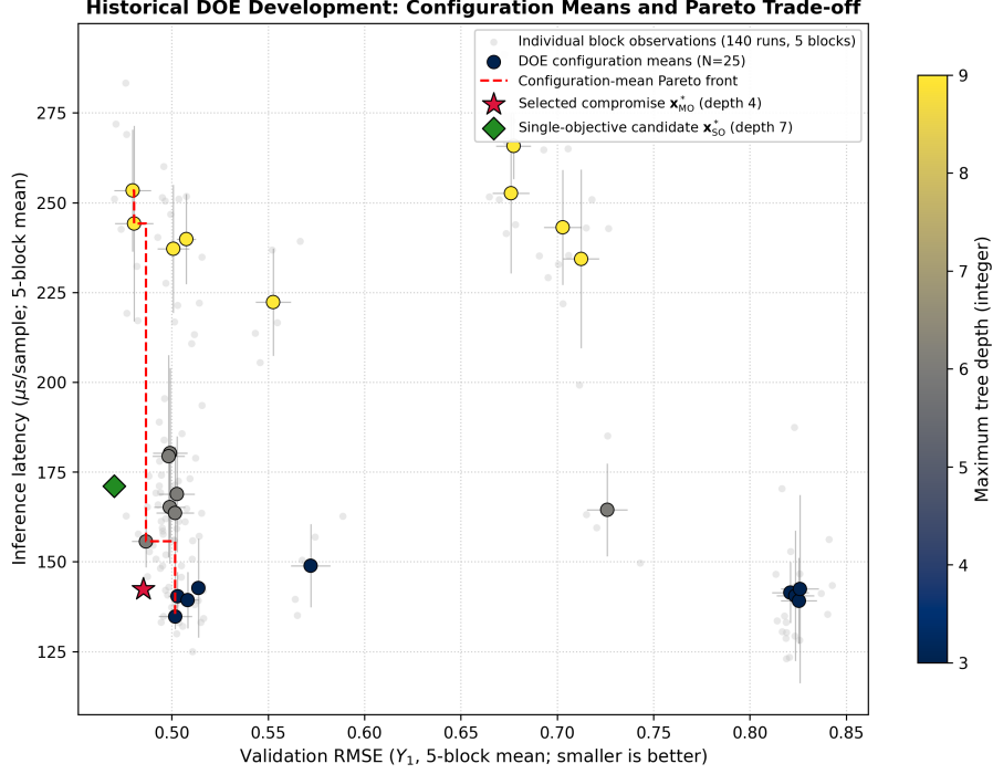
Figure 4: Historical DOE Multi-Objective Trade-Off: Validation RMSE vs. Inference Latency across 5 Seed Blocks. Light gray points show individual block run observations (140 runs across 5 blocks). Filled markers show the 25 unique design configuration means (averaged over blocks) colored by tree depth, with error bars indicating \pm 1 SD across blocks. The red dashed line traces the configuration-mean Pareto front. Highlighted operating coordinates include the multi-objective compromise \mathbf{x}_{\text{MO}}^* (depth 4, red star), single-objective candidate \mathbf{x}_{\text{SO}}^* (depth 7, green diamond), and empirical confirmation means ( m = 10 seeds).
