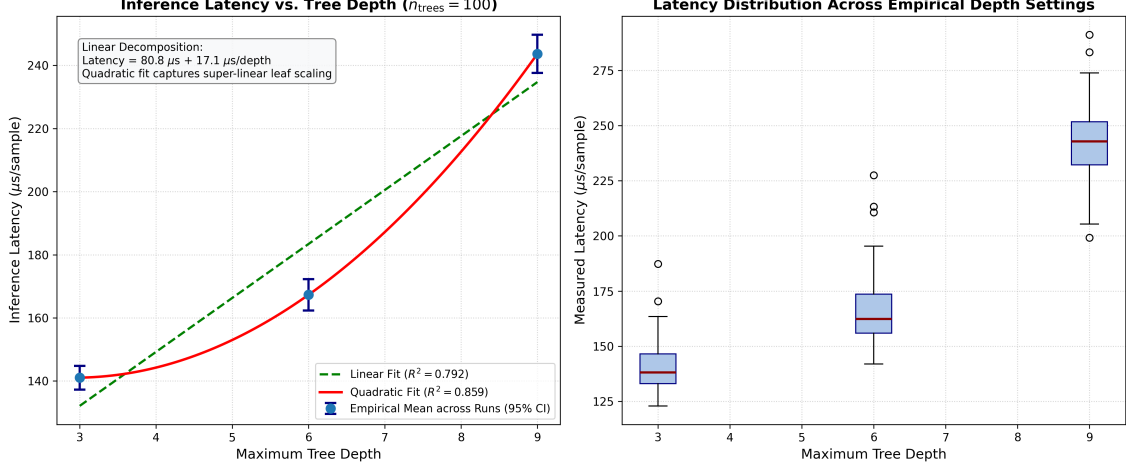
Figure 3: Inference Latency Modelling: (a) Empirical mean latency with 95% CI error bars vs. linear ( R^2 = 0.792 ) and quadratic ( R^2 = 0.859 ) fits. Note the linear base intercept ( \approx 80.8 \mu s ) arising from Python execution overhead; (b) Distribution boxplots across discrete depths.
