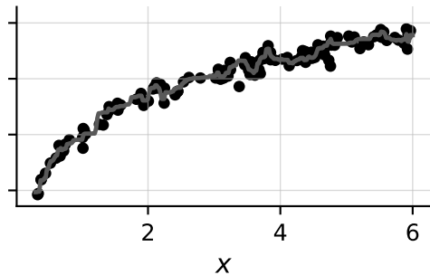
Random forest on x (RMSE 0.30)
