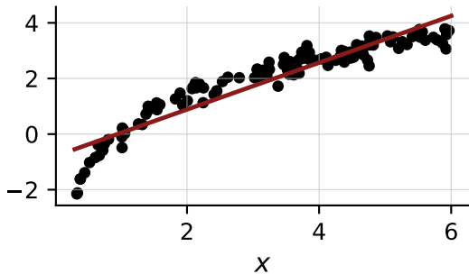
Least squares on x (RMSE 0.39)
