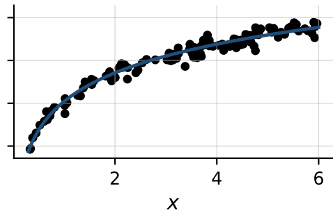
Least squares on \log x (RMSE 0.24)
