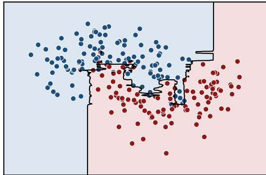
Average of 300 trees
