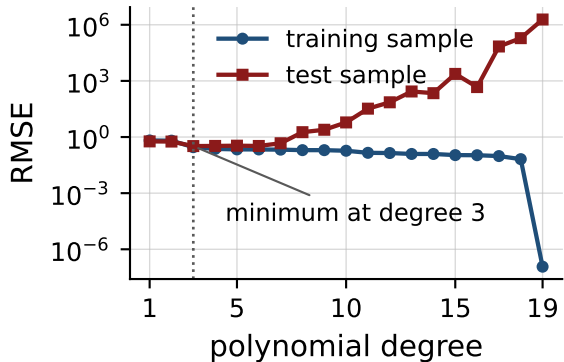
Training and test error
