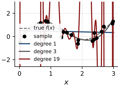
Fits to 20 observations
