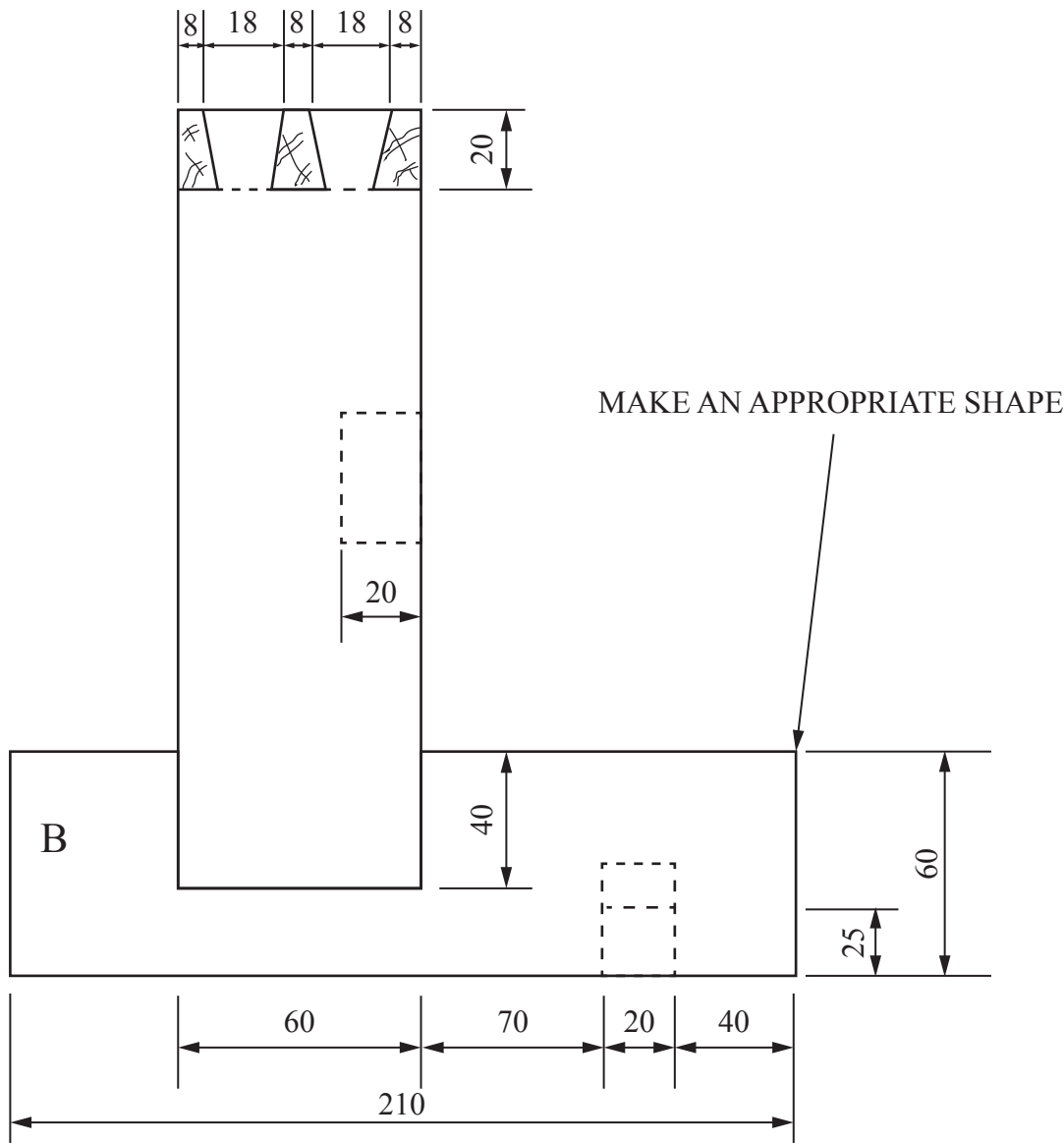
END VIEW
