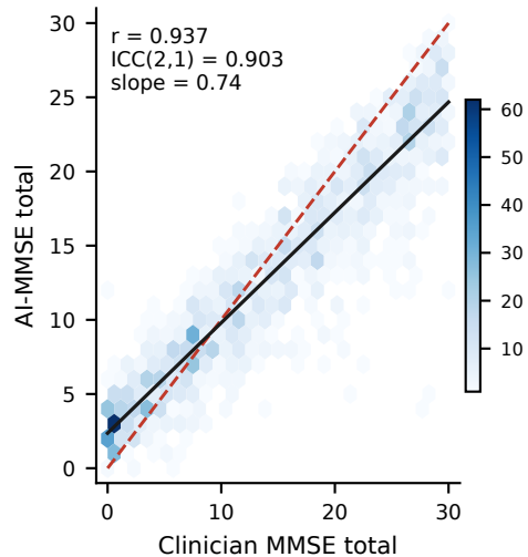
a Score agreement
