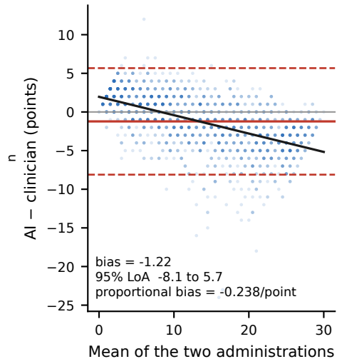
b Bland-Altman
