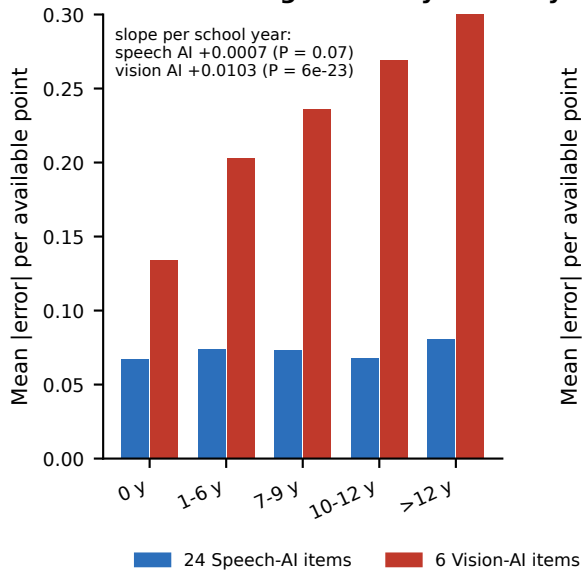
b Education gradient by modality
