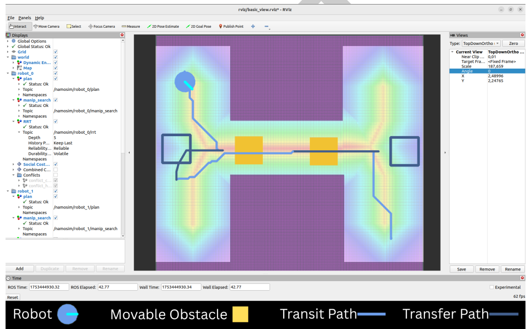
Figure 1: A NAMOSIM scenario with one robot and two obstacles is visualized in RViz. The robot's plan is shown by the blue lines. The darker shade of blue indicates the part of the path involving an obstacle transfer. The social costmap is seen in the rainbow background.
