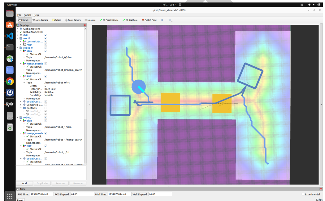
Figure 1: NAMOSIM
