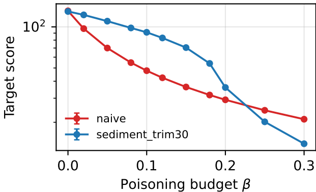
Target score under poisoning
