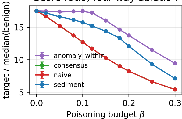
Score ratio, four-way ablation
