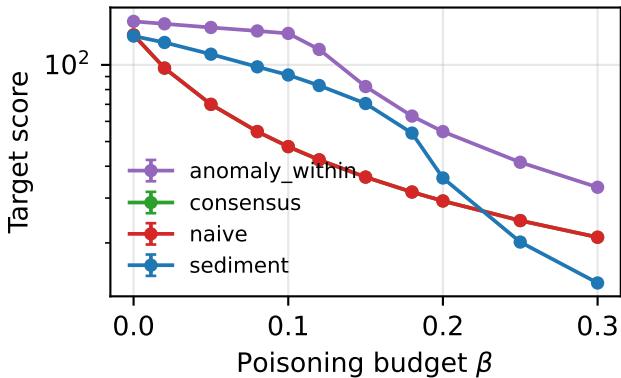
Target score, four-way ablation
