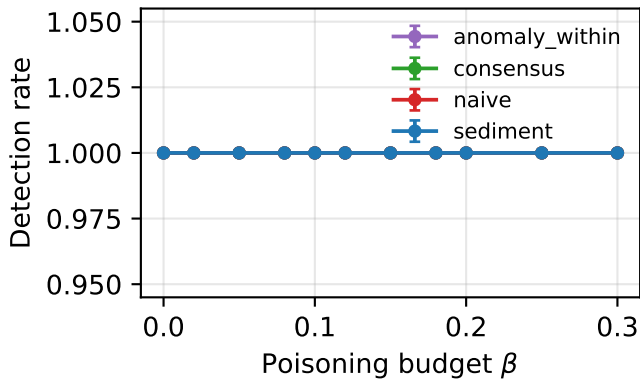
Detection rate at 5 percent FPR, white-box targeted attack
