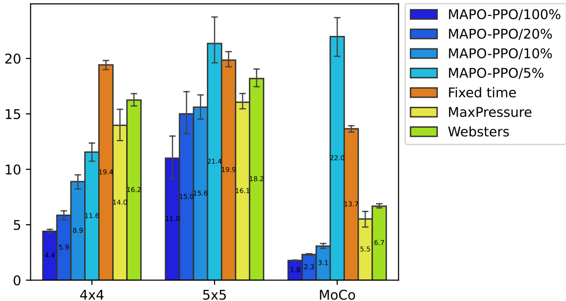
Average queue length (veh)
