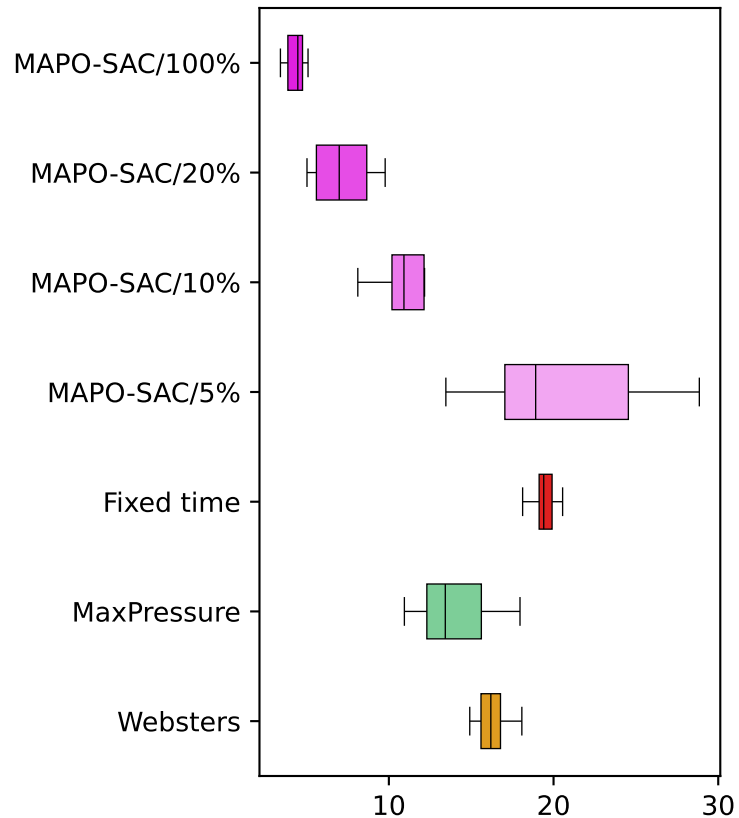
Average queue length (veh)
