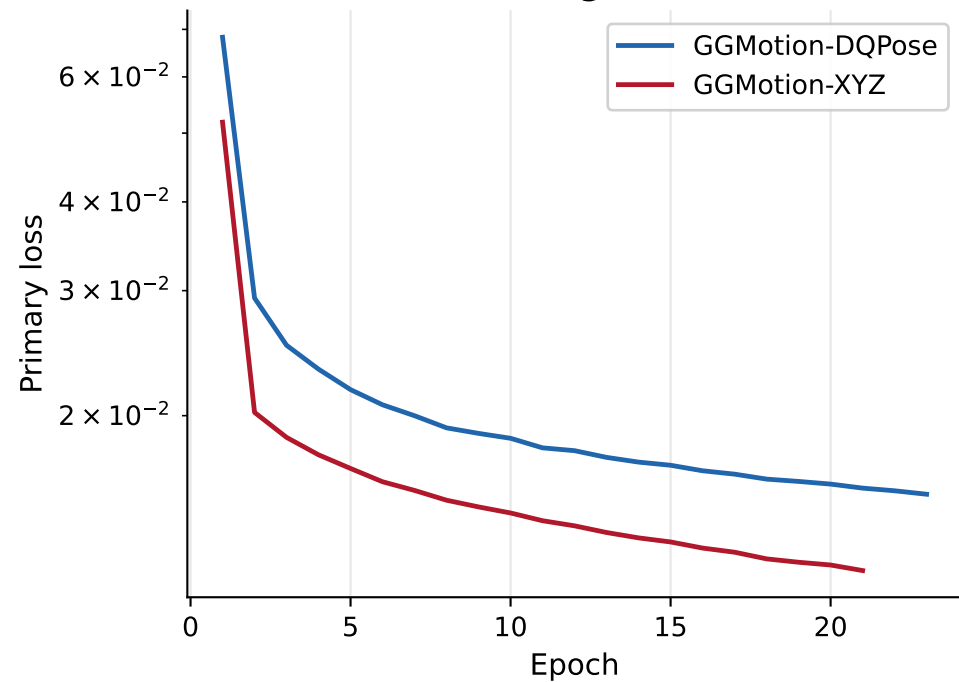
Training Loss
