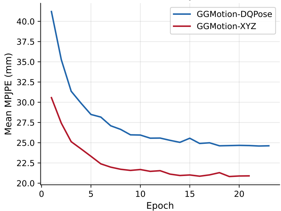
Validation MPJPE
