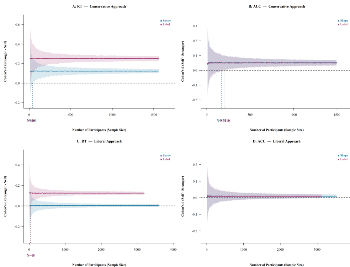
Figure 5. Bootstrap estimation of the self-prioritization effect under nonmatching conditions. A and B, the conservative approach; C and D, the liberal approach.
