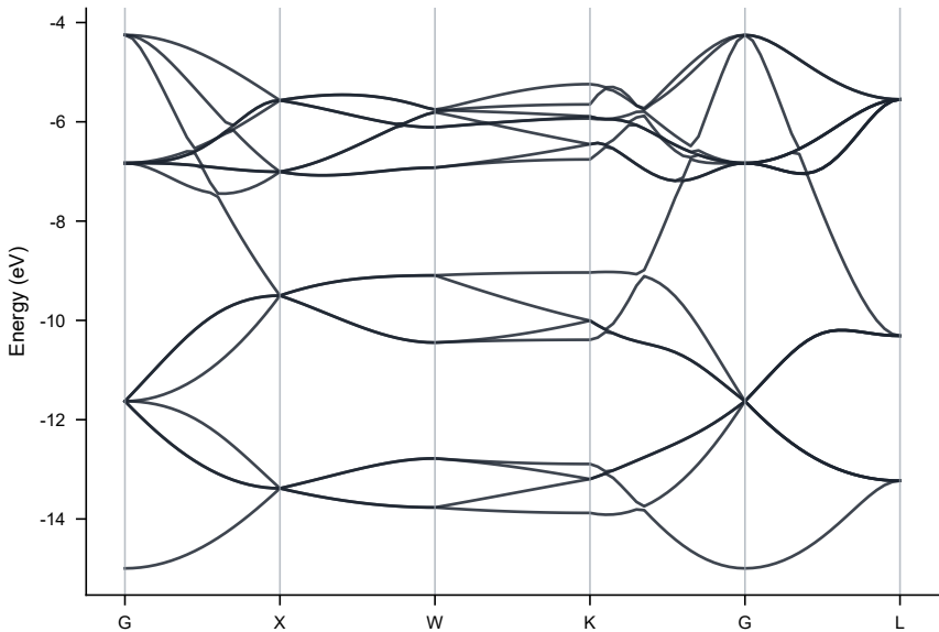
DFTB+ band structure
