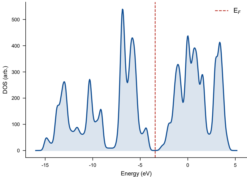
DFTB+ density of states (from band path)
