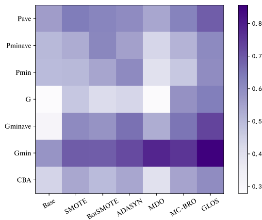
Fig. 8 The mean results of all methods on different metrics (datasets 1–15)
