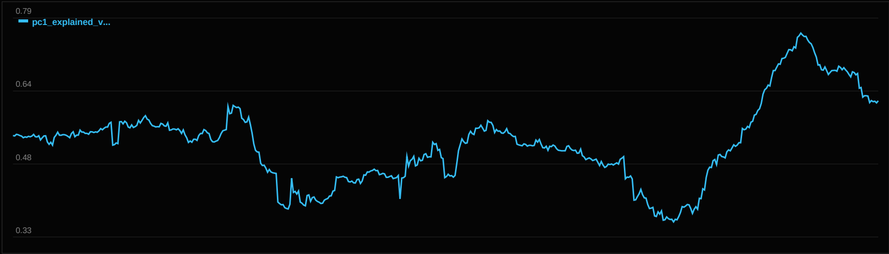
ROLLING PC1 EXPLAINED VARIANCE
