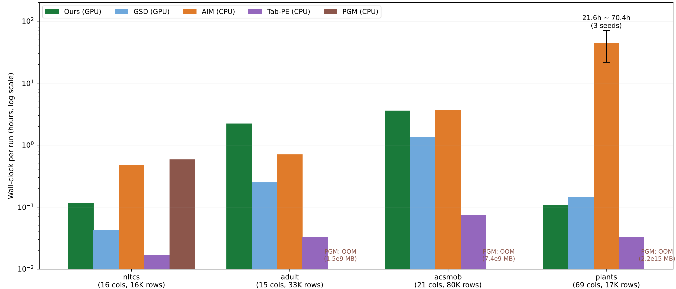
Wall-clock comparison at \varepsilon = 1 (noisy runs, mean of 3 seeds)
