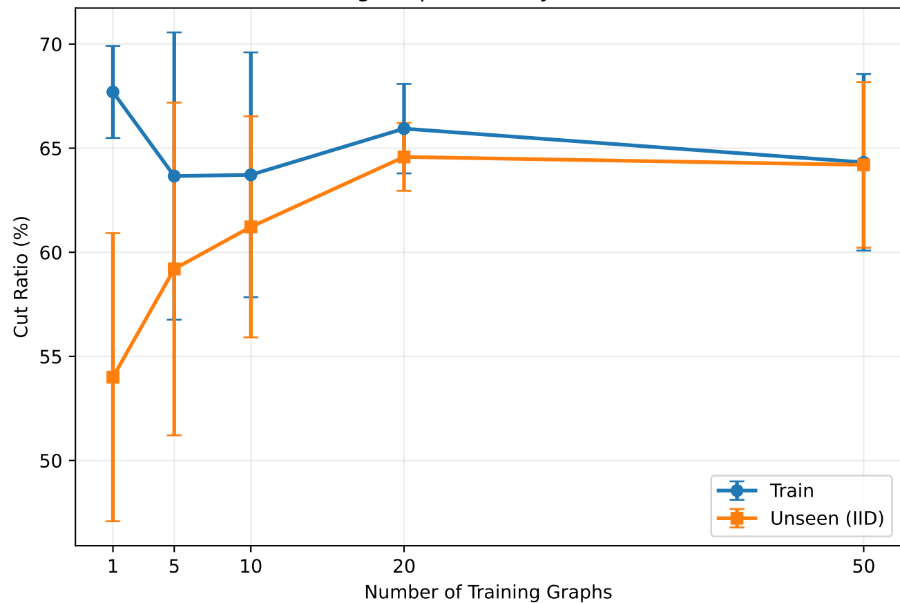
Effect of Training-Graph Diversity on IID Generalization
