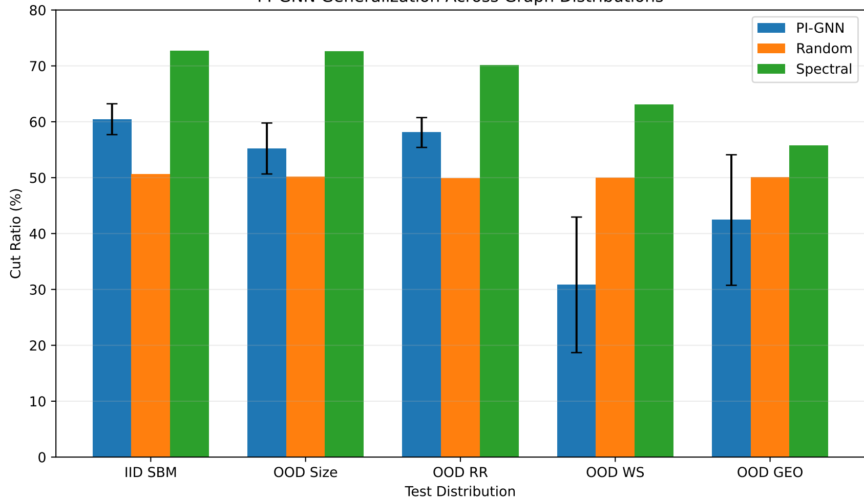
PI-GNN Generalization Across Graph Distributions
