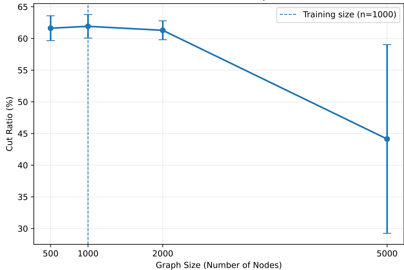
Generalization Across Graph Sizes
