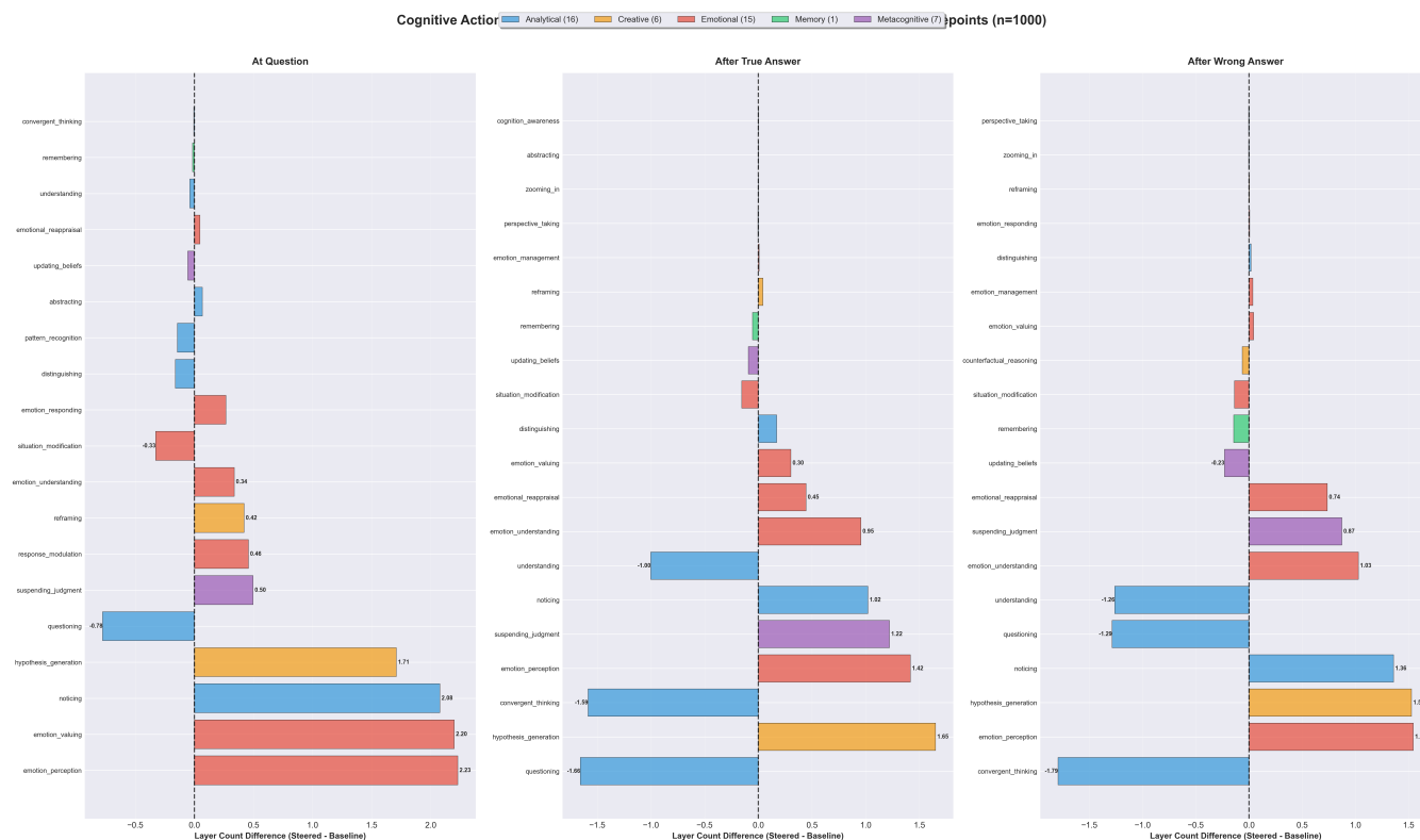
Figure 1: Steering effects across all cognitive actions and timepoints (n=1000). Left panels show individual action changes at three timepoints: at question (before answer), after true answer, and after wrong answer. Bars indicate mean layer count difference (steered - baseline) with positive values (right) showing increases and negative values (left) showing decreases. Emotional actions ( emotion_perception , emotion_valuing , noticing ) consistently increase across timepoints, while analytical actions ( questioning , convergent_thinking , understanding ) consistently decrease, revealing the emotional foundation of successful ToM.
