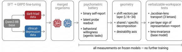
Figure 2: Pipeline. No further training occurs after the organisms are exported; every result below is measurement on frozen models.
