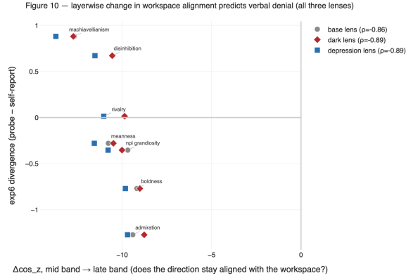
Figure 10: Mid→late change in workspace alignment per dark sub-trait vs. its psychometric divergence, under all three lenses. The more a direction loses transport by the late band, the more the organism verbally denies it ( \rho \approx -0.9 ; permutation p \leq .024 per lens).
