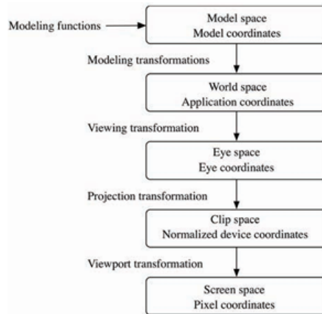
Hình 1.1: Vertex processing in the OpenGL pipeline [8]
