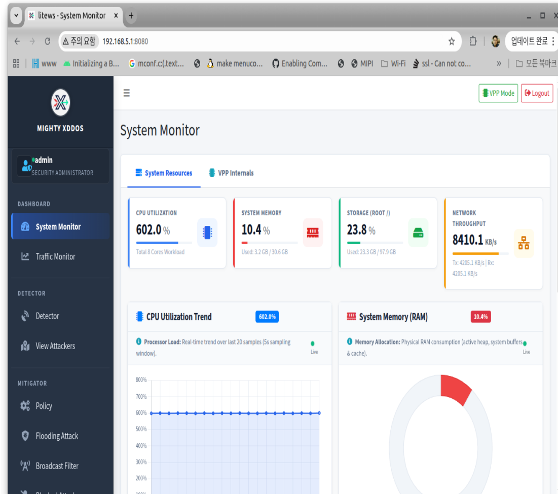
DashBoard – System Monitor Page
