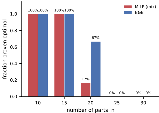
b exact reach by size
