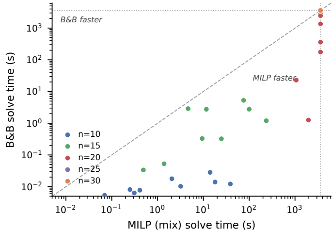
a head-to-head (same 3600 s limit)
