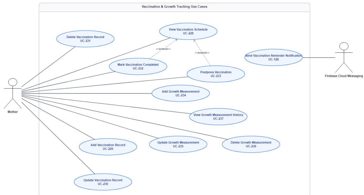
Figure 31: Vaccination & Growth Tracking Use Cases
