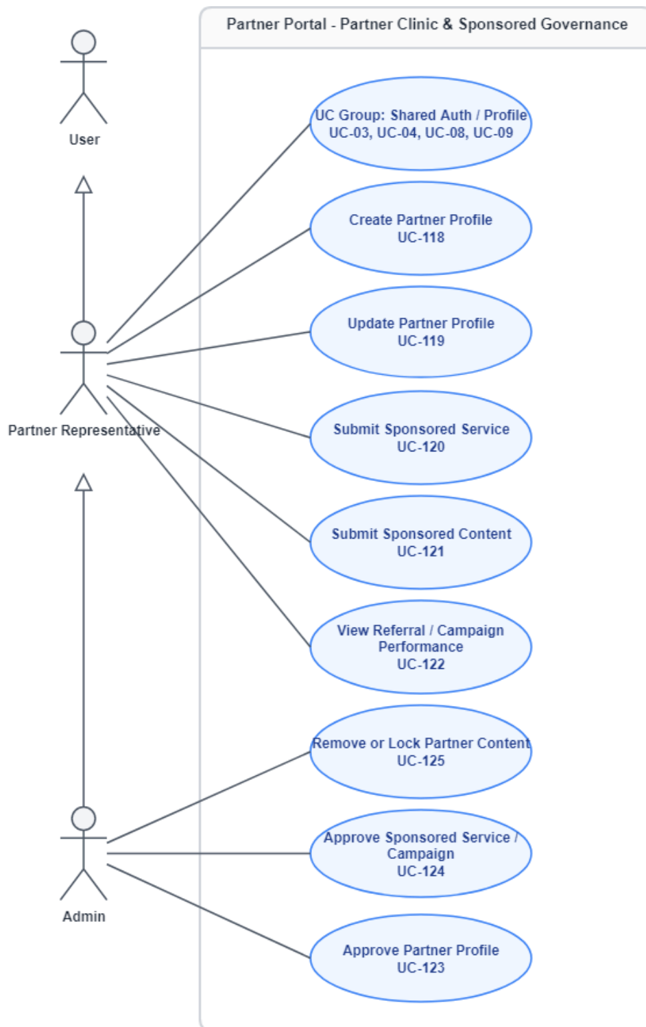
Figure 22: Partner Use Cases
