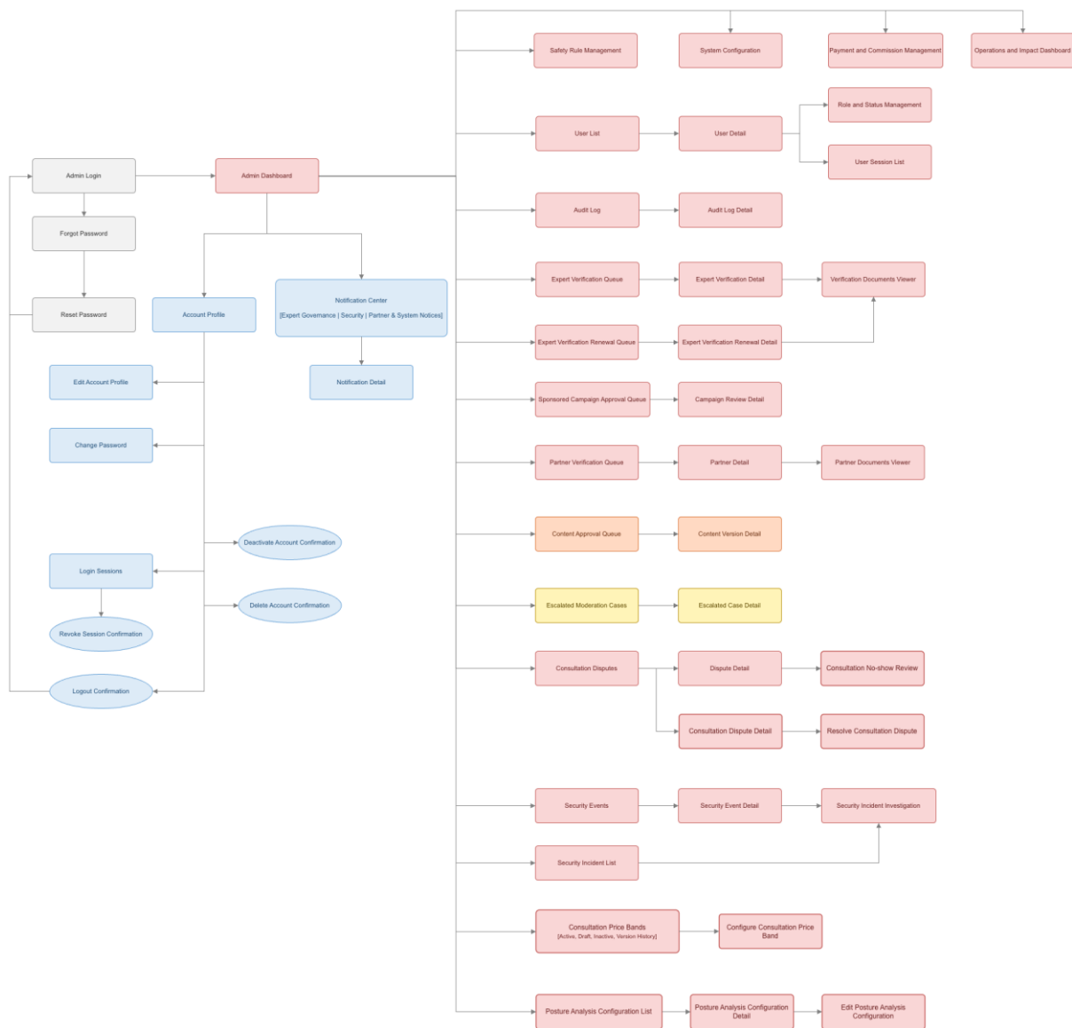
Figure 37: System Admin Web Portal Screens Flow
