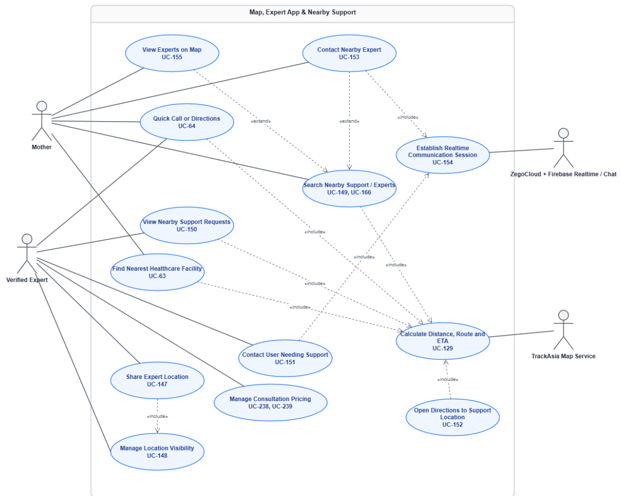
Figure 26: Map, Expert App & Nearby Support Use Cases
