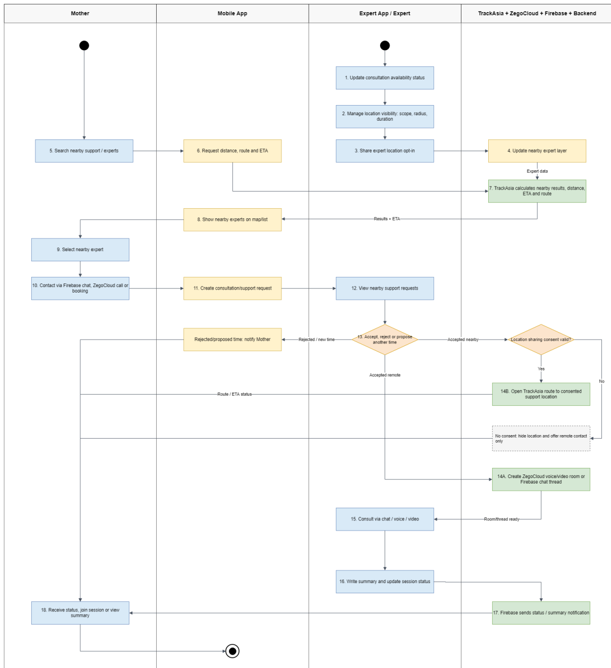
Figure 11: Expert App, TrackAsia Nearby Support & Realtime Contact Workflow
