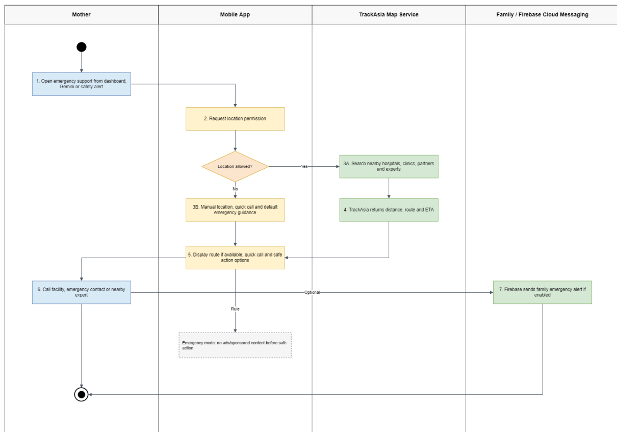
Figure 8: TrackAsia Emergency Map & Nearby Care Workflow
