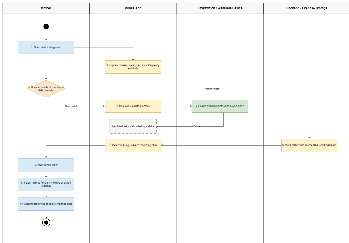
Figure 13: Smartwatch Data Sync & Health Trend Workflow
