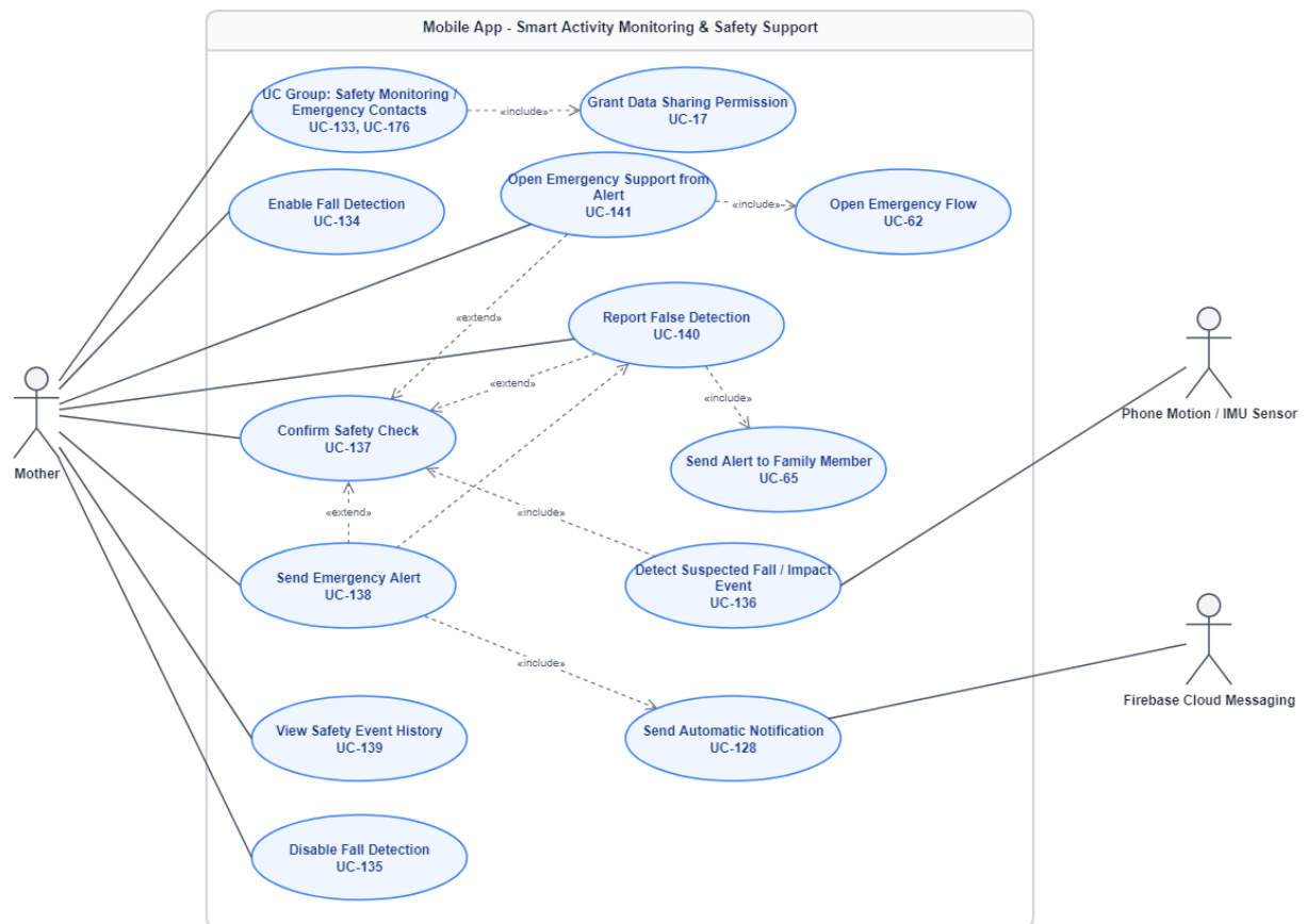
Figure 24: Smart Activity Monitoring & Safety Support Cases
