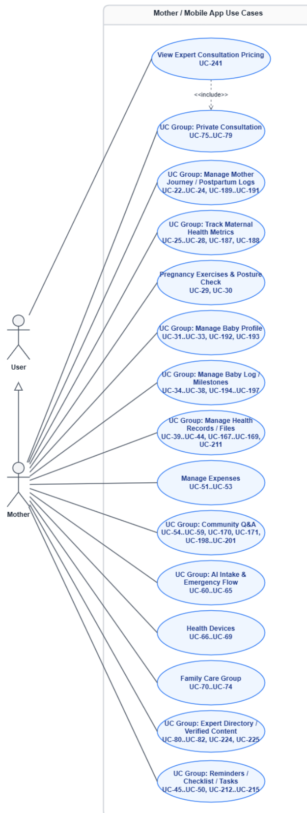
Figure 18: Mother Use Cases
