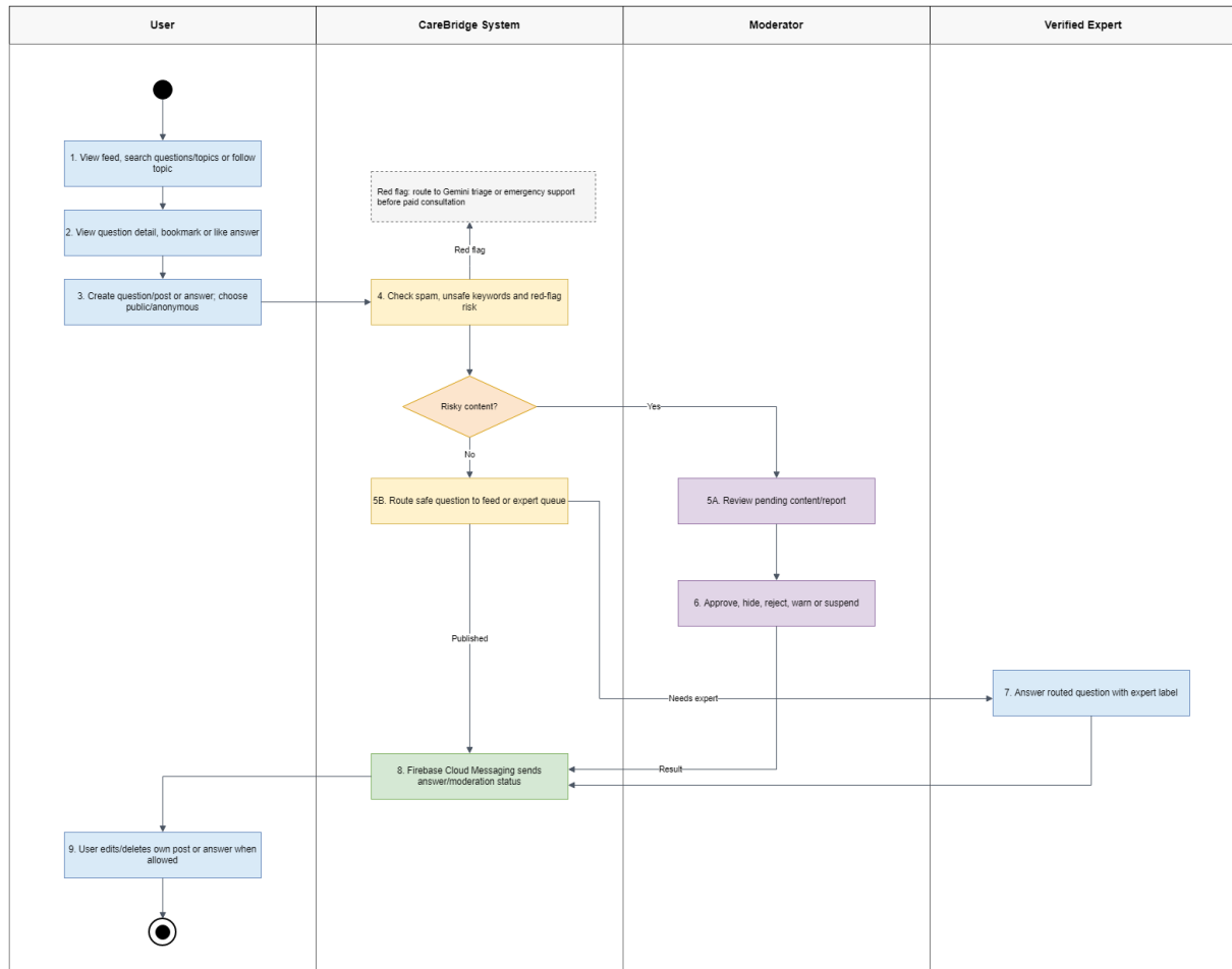
Figure 5: Community Q&A, Expert Answer & Moderation Workflow
