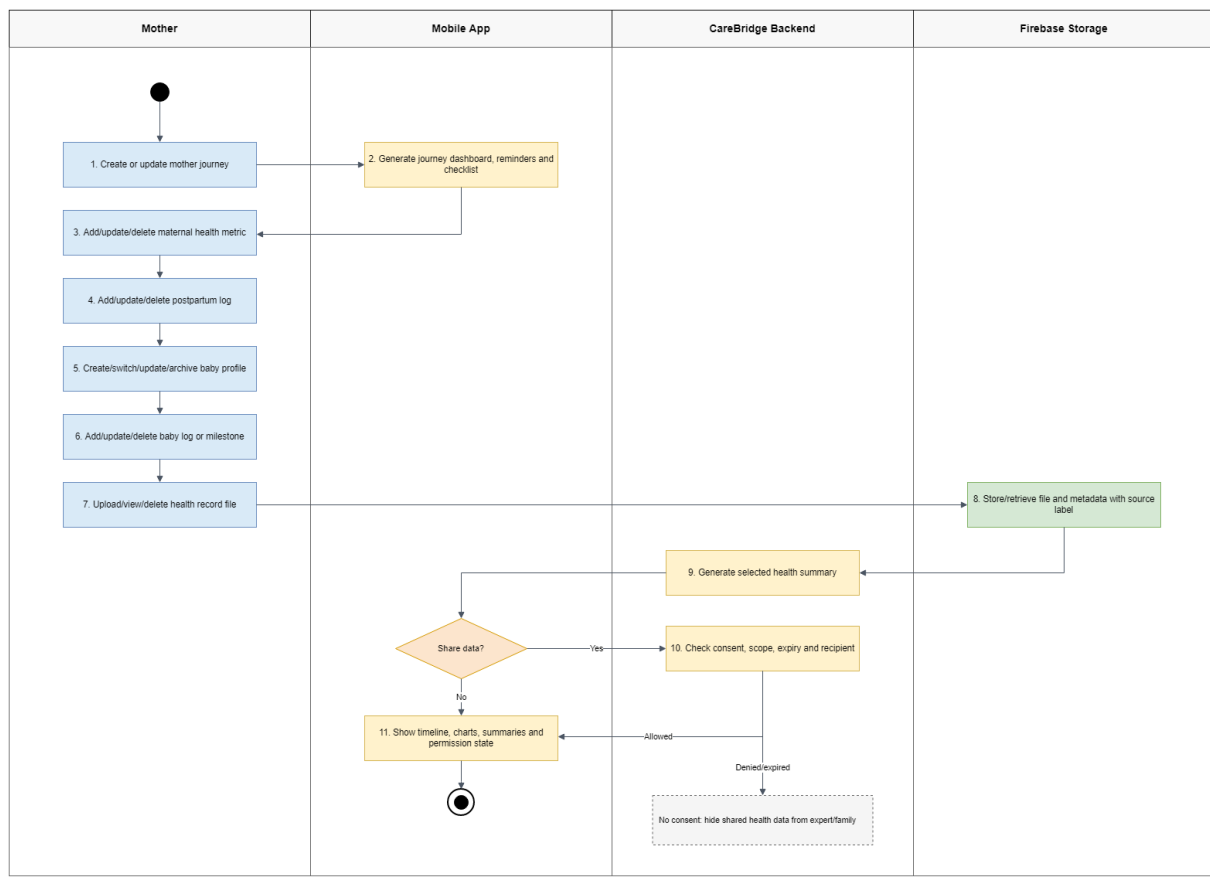
Figure 4: Mother, Baby & Health Record Workflow
