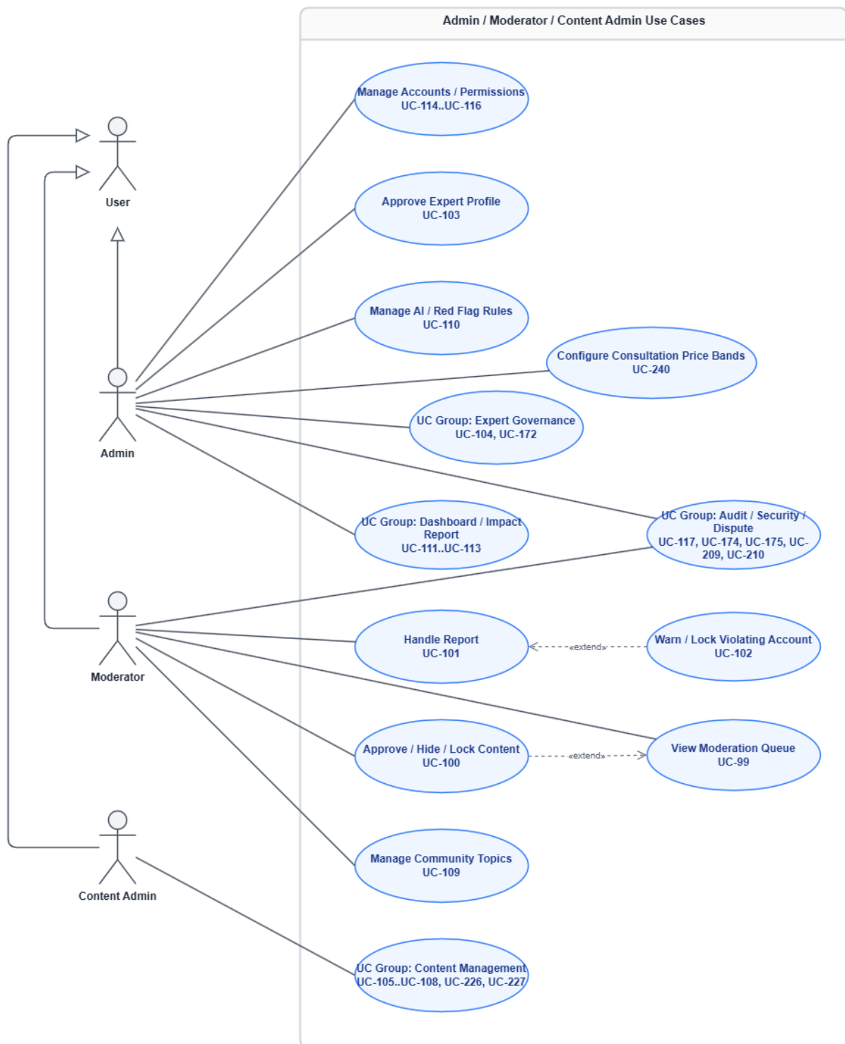
Figure 21: Content, Moderation & Operations Use Cases
