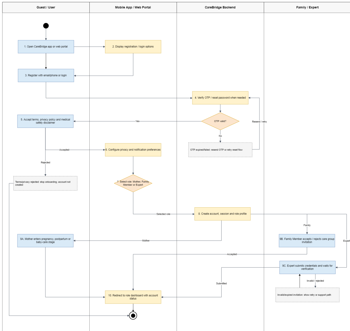
Figure 3: User Onboarding, Account & Privacy Setup Workflow
