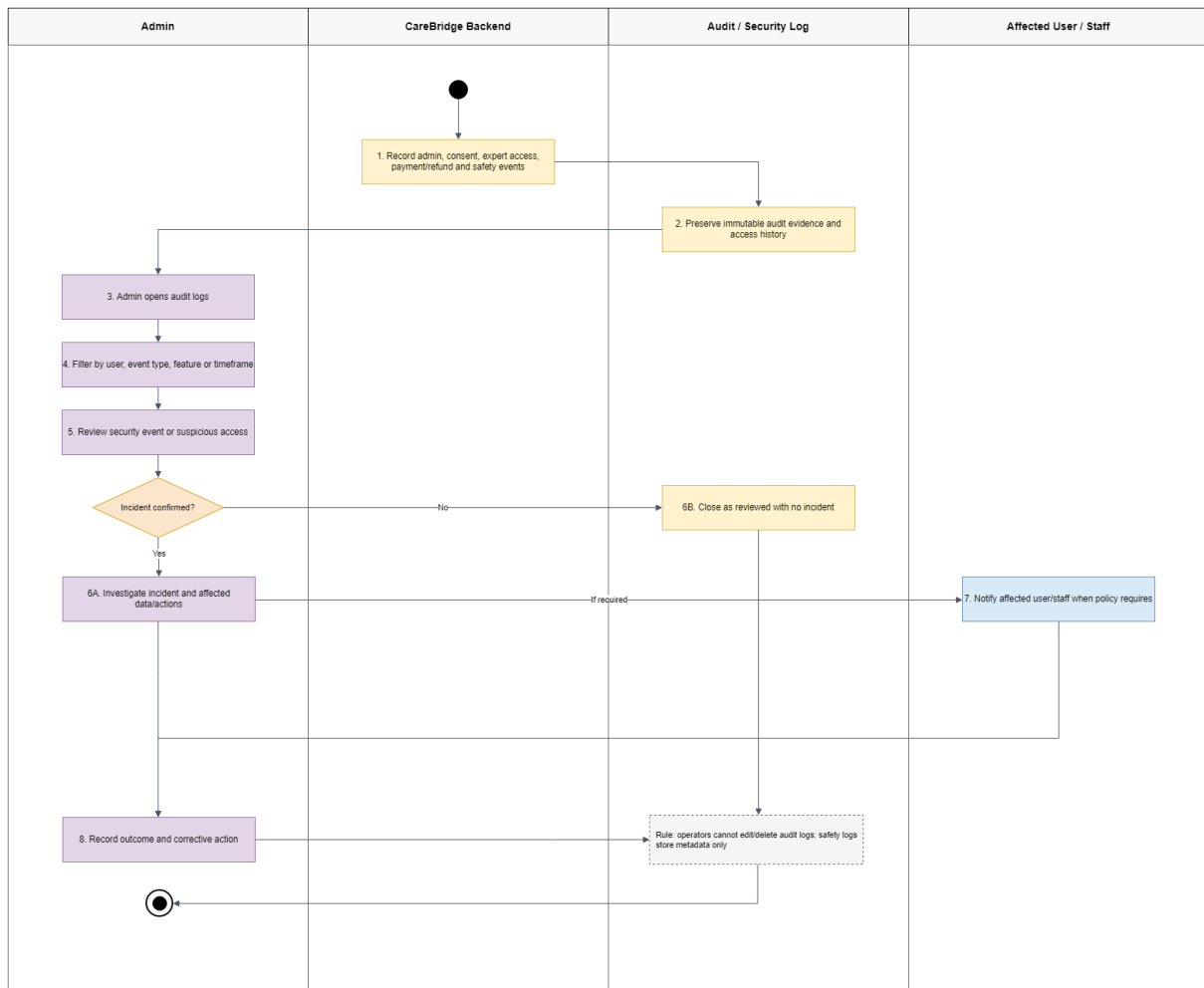
Figure 16: Audit, Security Incident & Access Review Workflow
