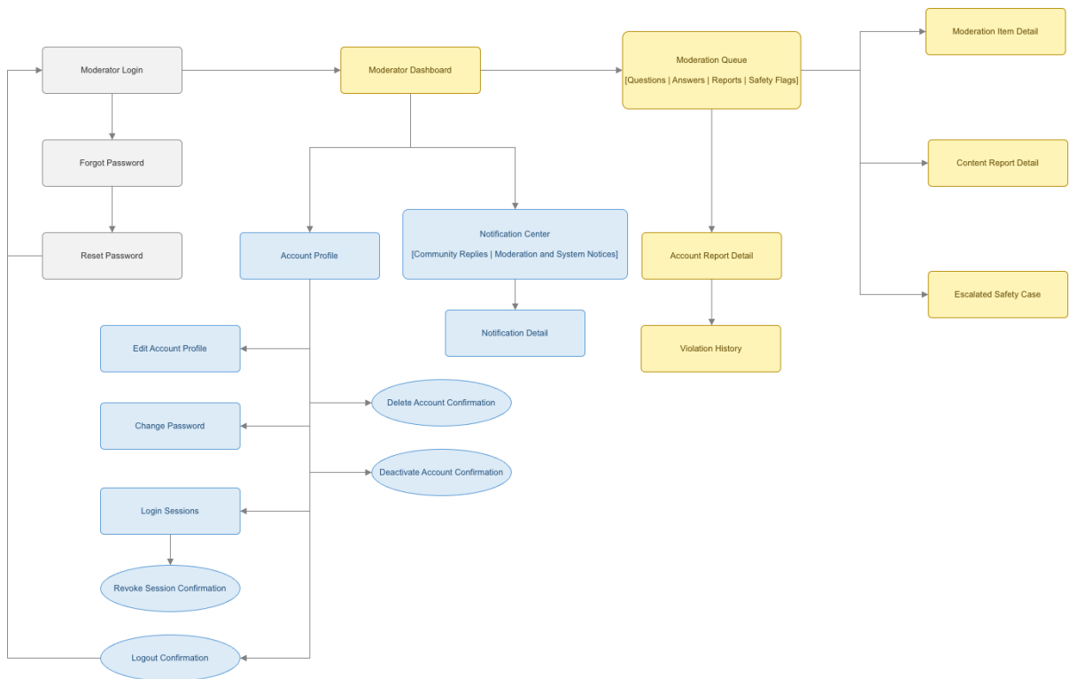
Figure 39: Moderator Web Portal Screens Flow
