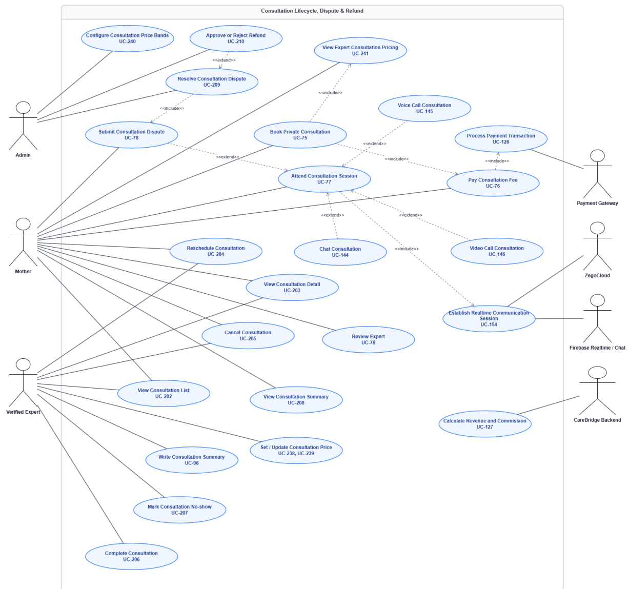
Figure 28: Consultation Lifecycle, Dispute & Refund Use Cases
