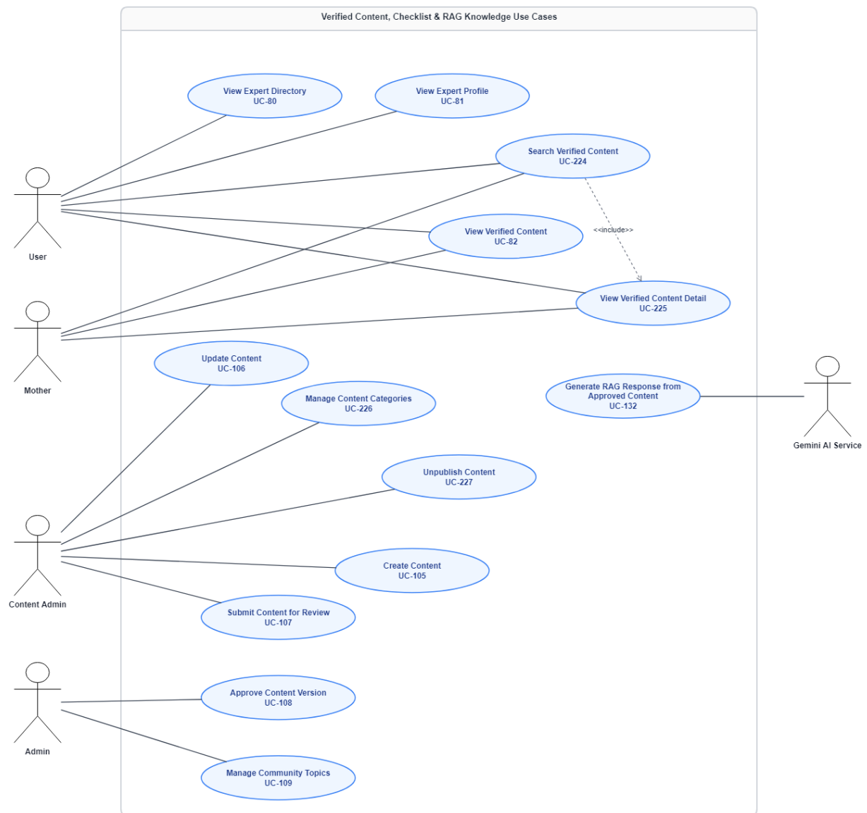
Figure 30: Verified Content, Checklist & RAG Knowledge Use Cases
