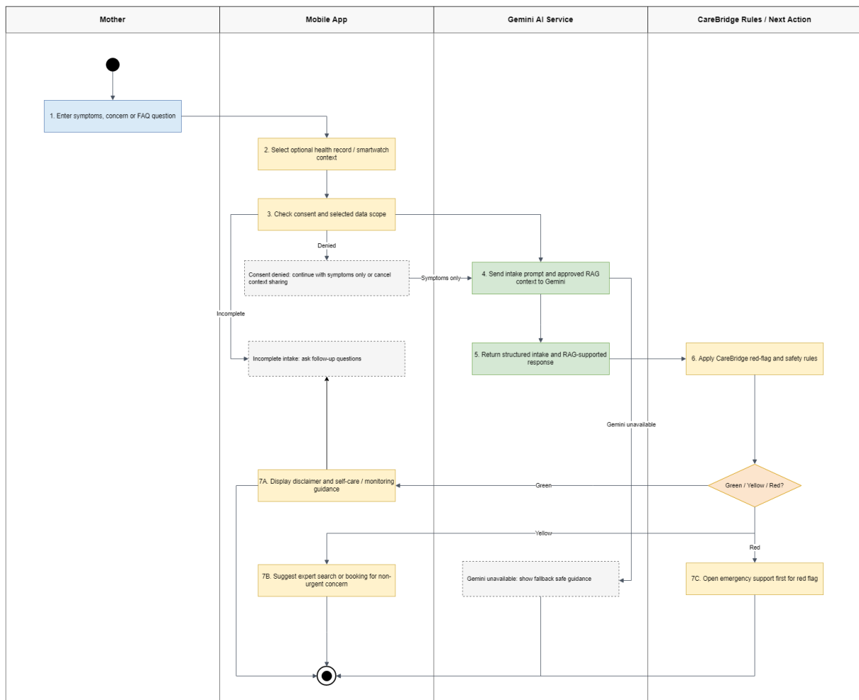
Figure 7: Gemini AI Triage & Safe Action Workflow
