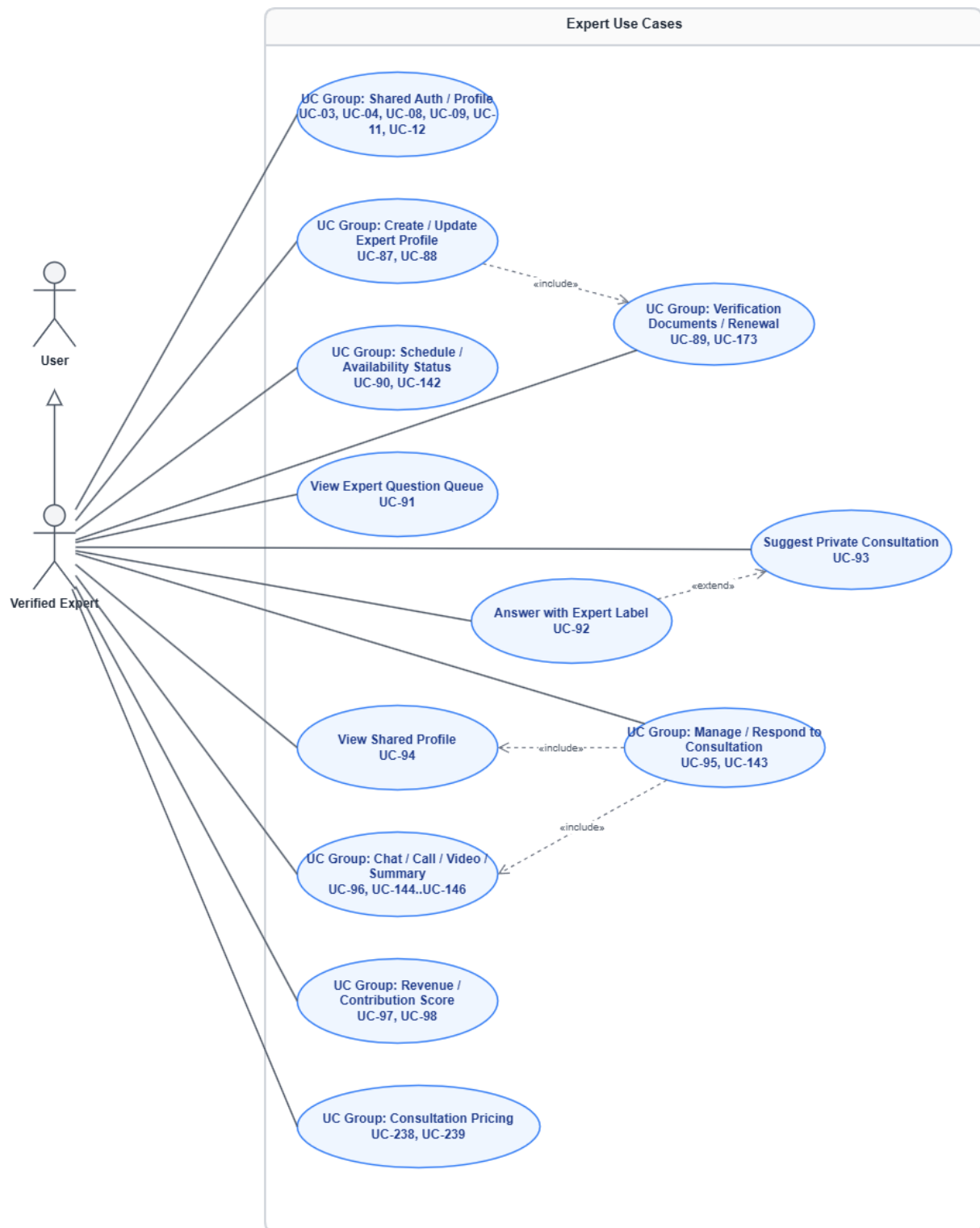
Figure 20: Expert Use Cases
