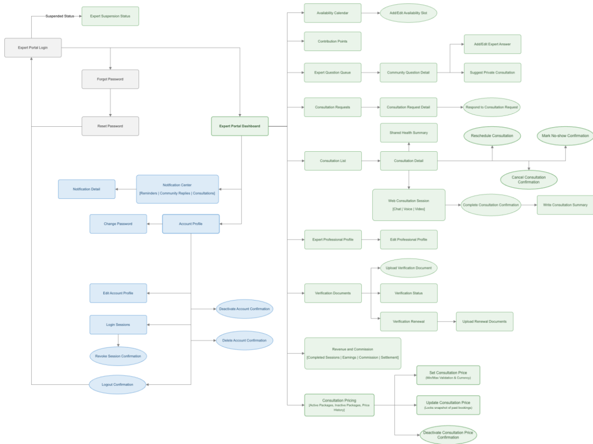
Figure 36: Verified Expert Web Portal Screens Flow
