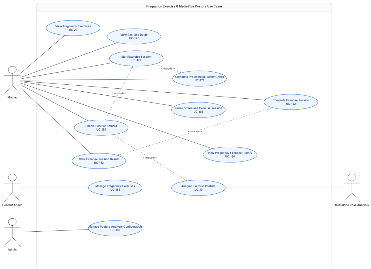
Figure 27: Pregnancy Exercise & MediaPipe Posture Use Cases
