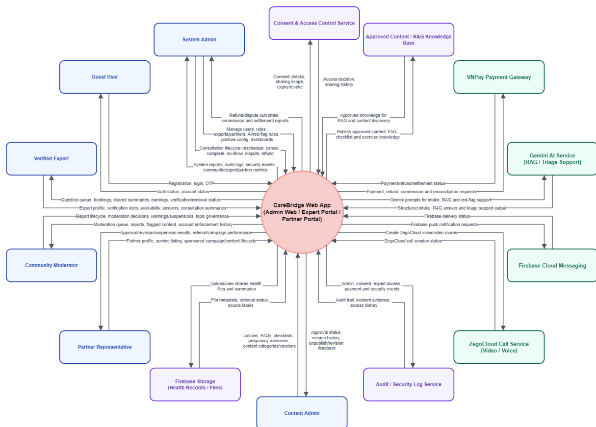
Figure 1: Context Diagram for Web App
