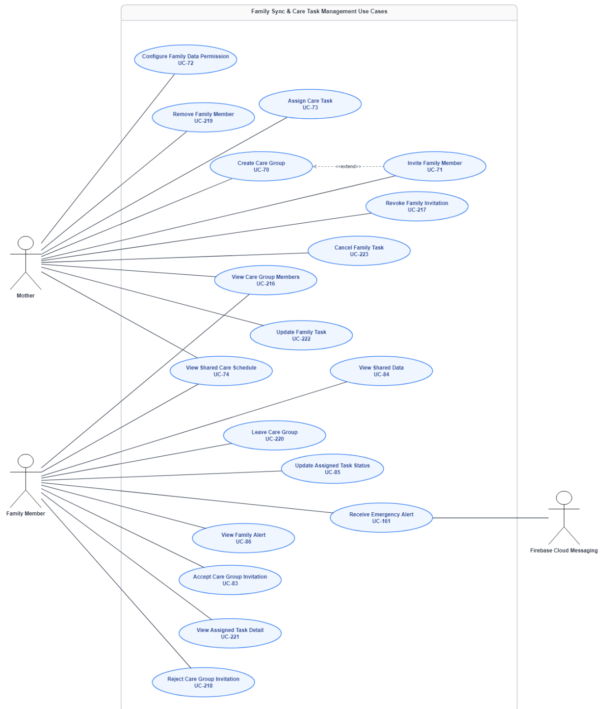
Figure 29: Family Sync & Care Task Management Use Cases
