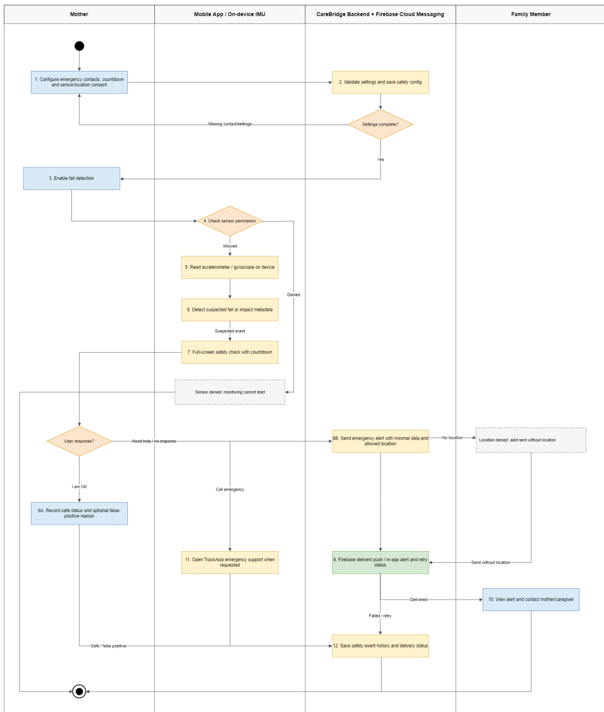
Figure 10: Smart Activity Monitoring & Safety Support Workflow
