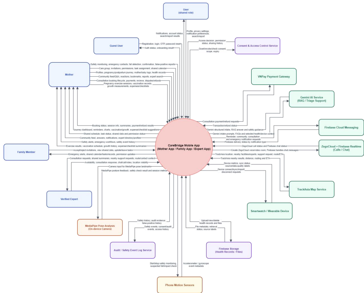
Figure 2: Context Diagram for Mobile App
