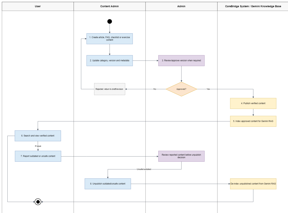
Figure 15: Verified Content, Checklist & Gemini RAG Knowledge Workflow
