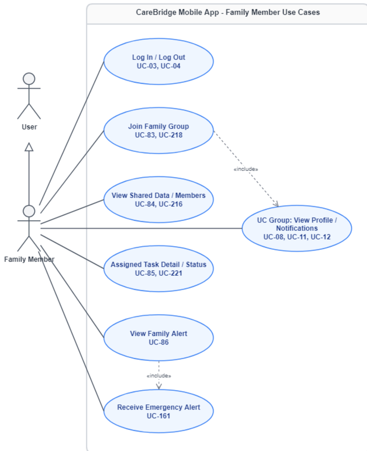
Figure 19: Family Member Use Cases
