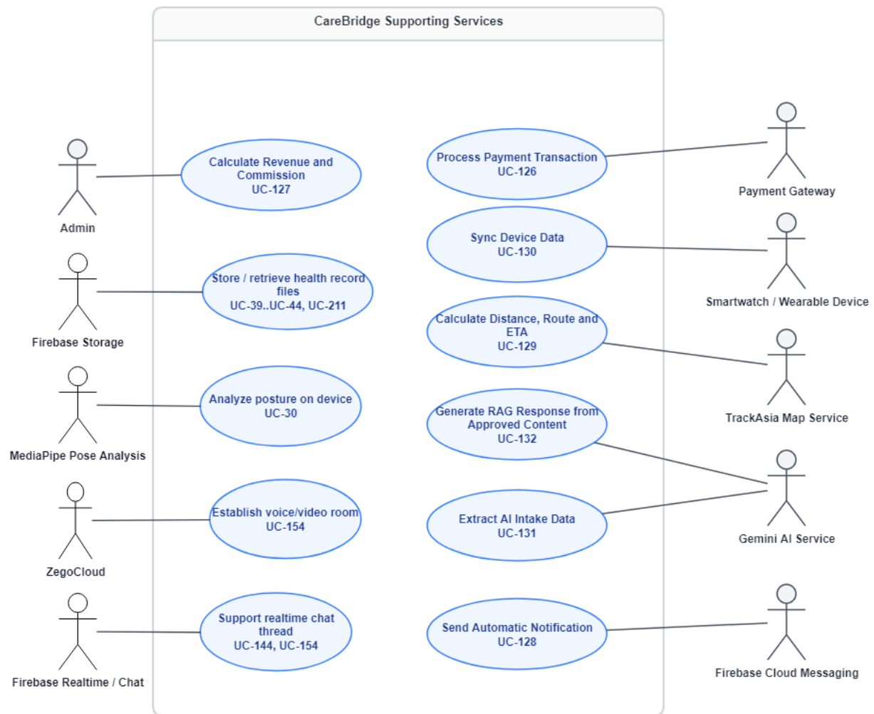
Figure 23: Supporting Services Use Cases
