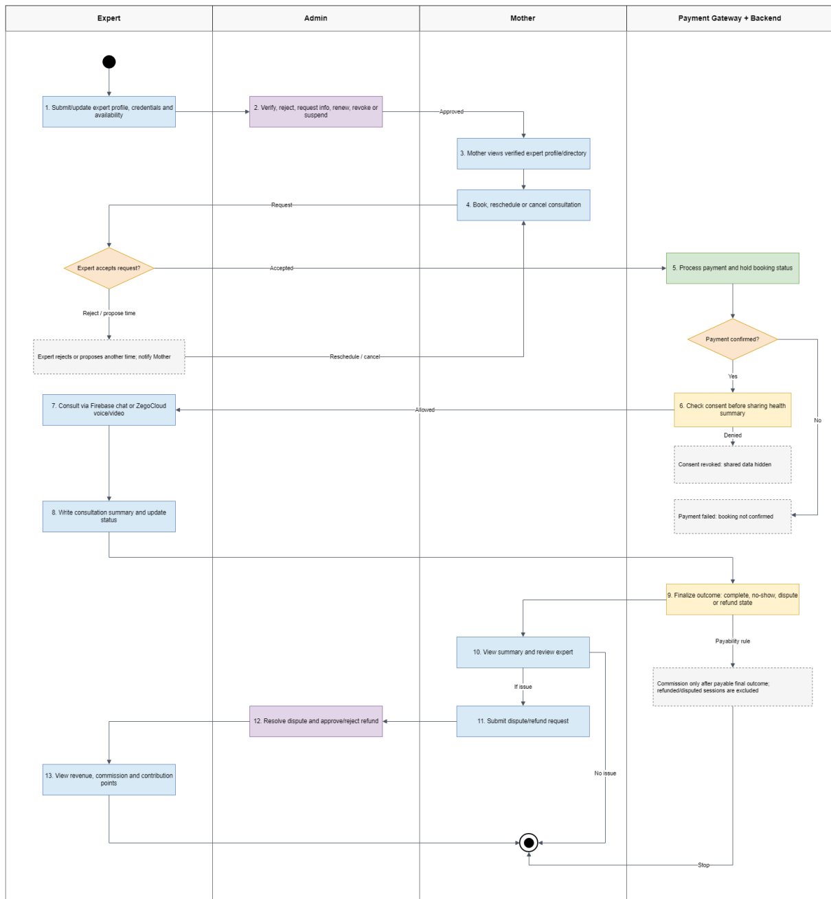
Figure 6: Expert Verification, Booking & Consultation Workflow
