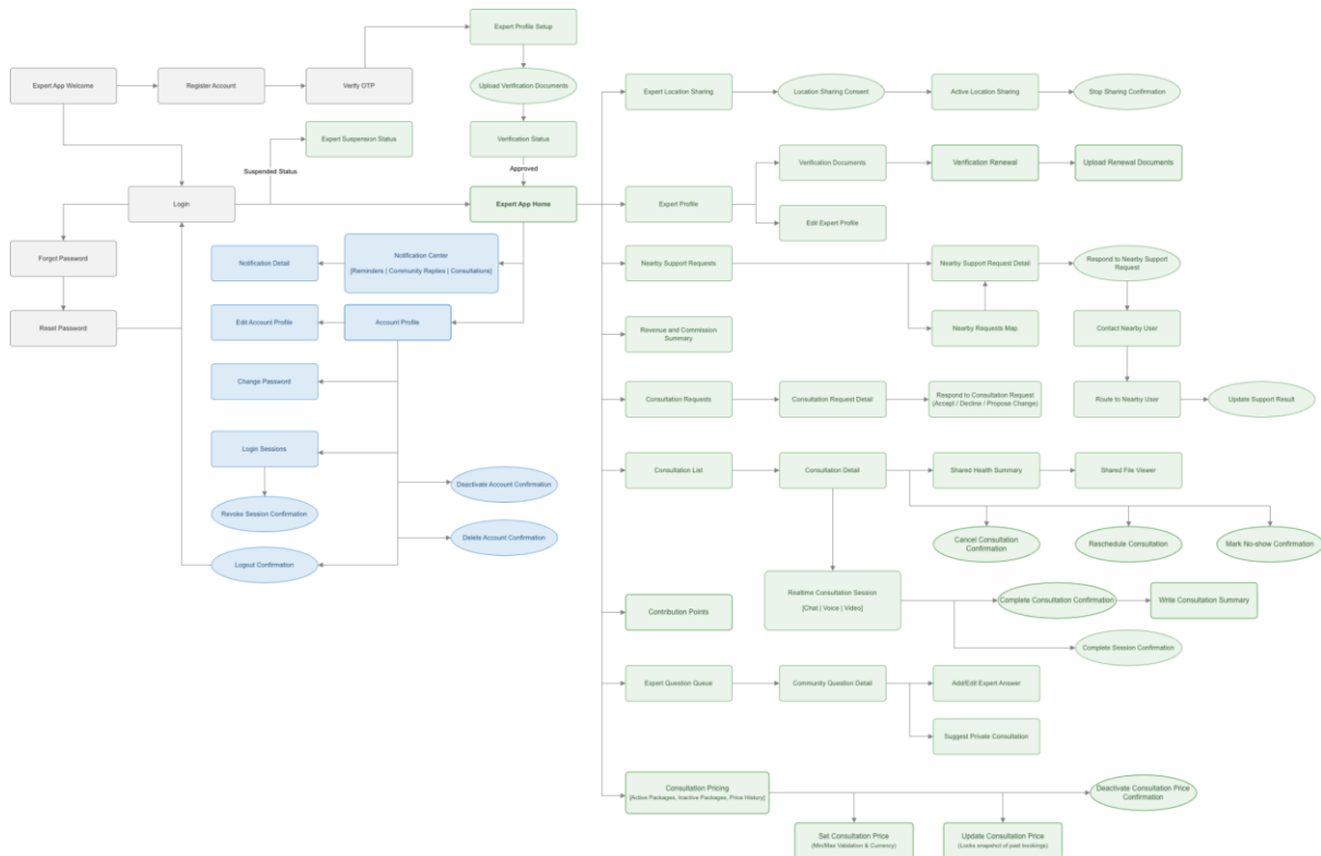
Figure 35: Verified Expert App Screens Flow
