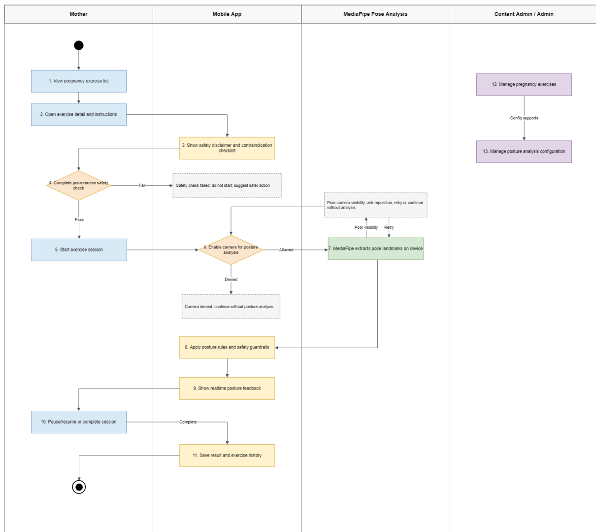
Figure 12: Pregnancy Exercise & MediaPipe Posture Workflow
