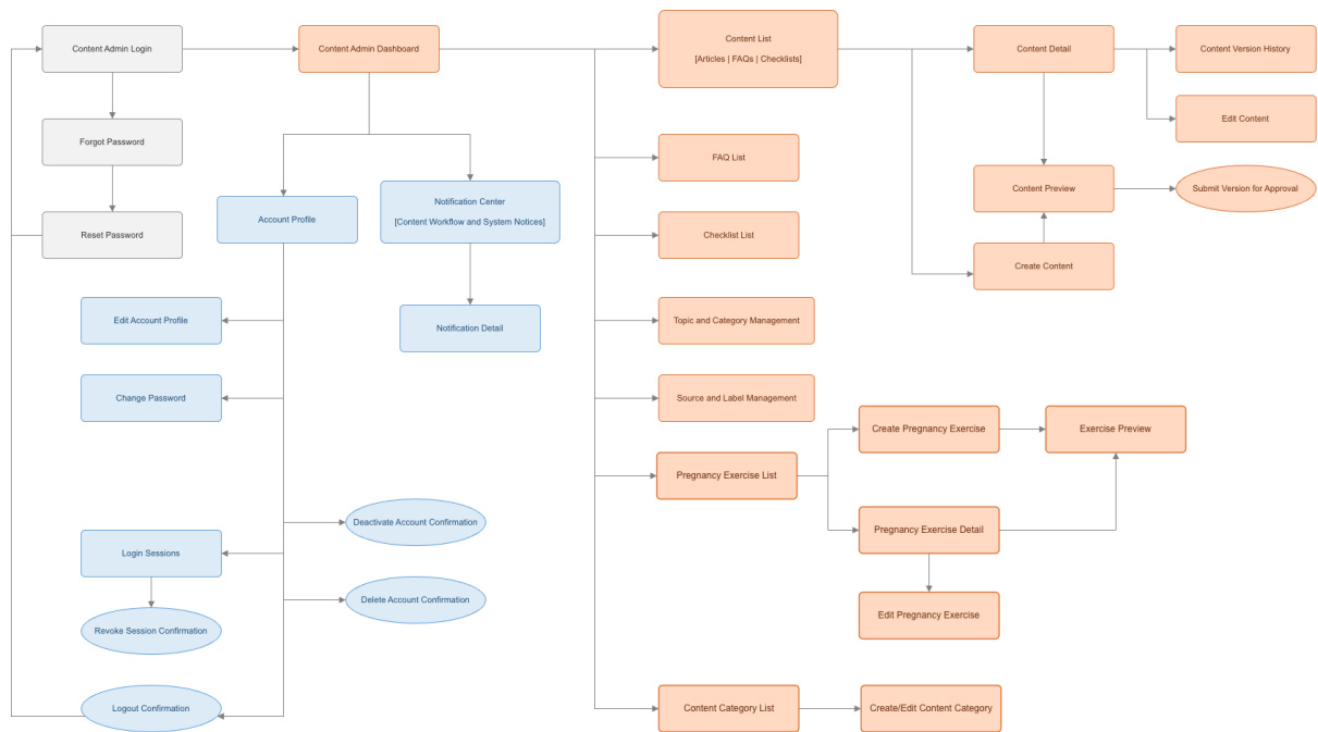
Figure 38: Content Admin Web Portal Screens Flow
