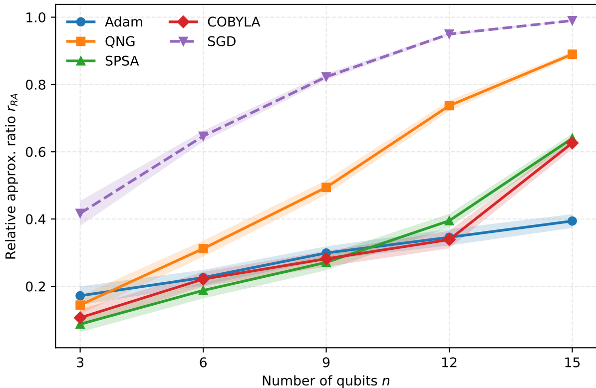
IQP full connectivity, Ising, L = 1 , \mathcal{N}(0, 1) init (50 instances)
