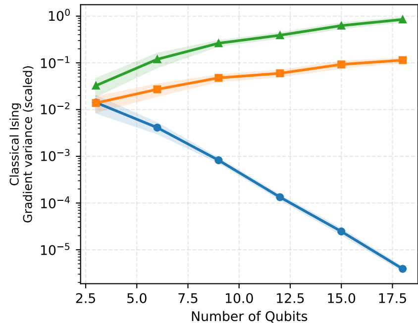
Normal (0, 1)
