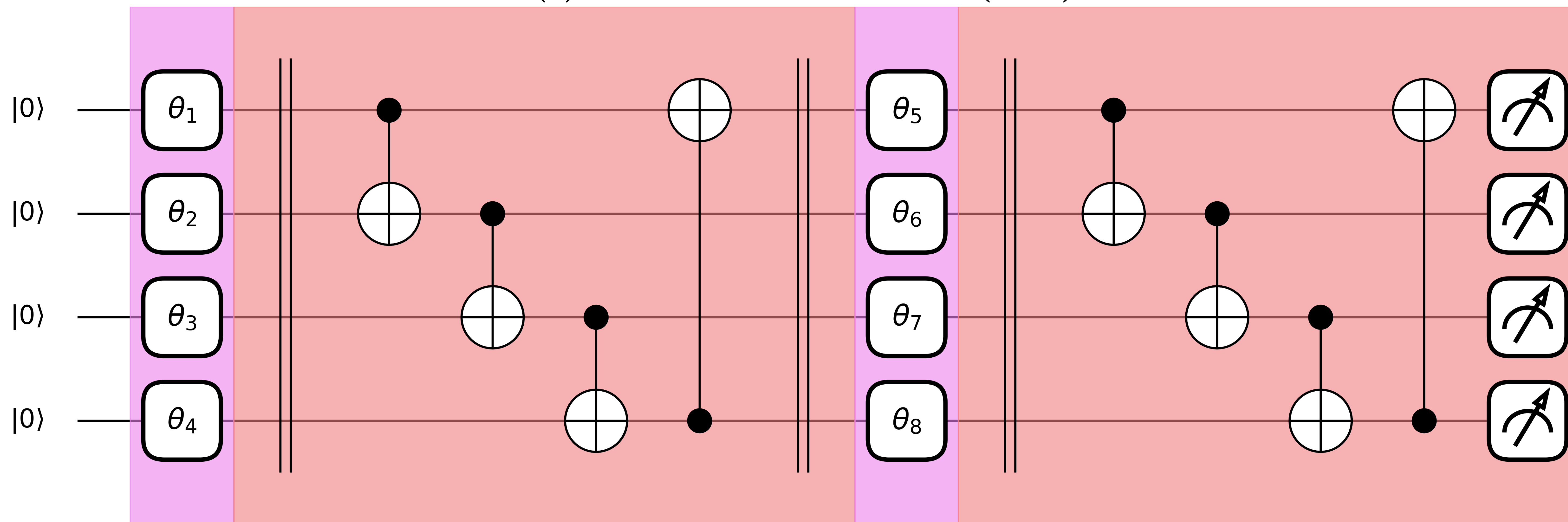
(a) Hardware Efficient Ansatz ( L = 2 )
