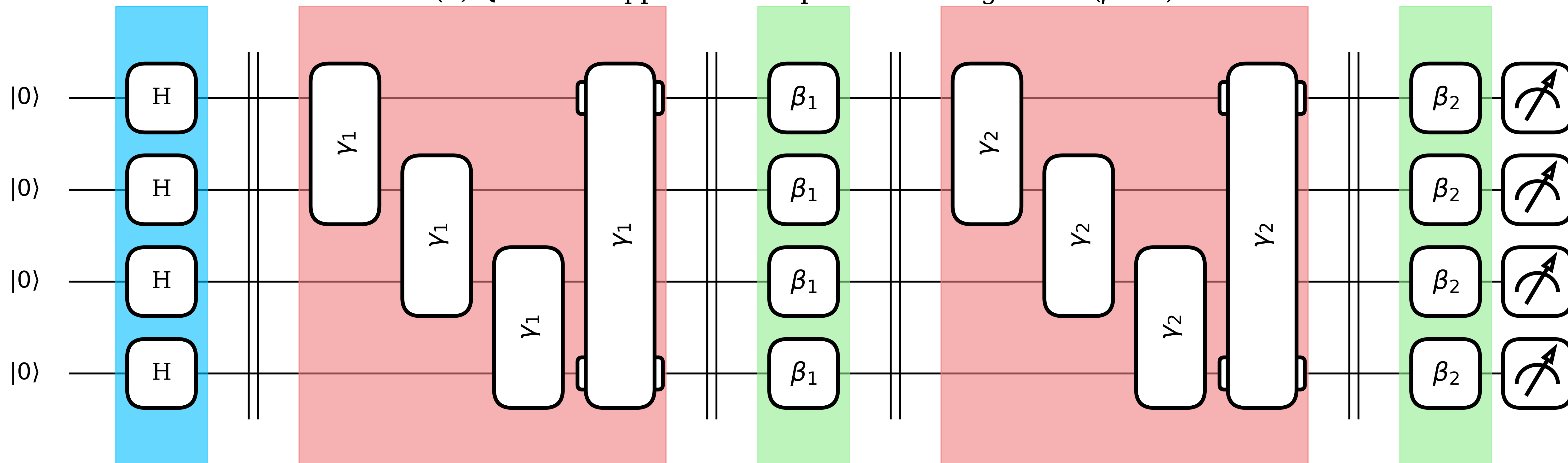
(b) Quantum Approximate Optimization Algorithm ( p = 2 )
