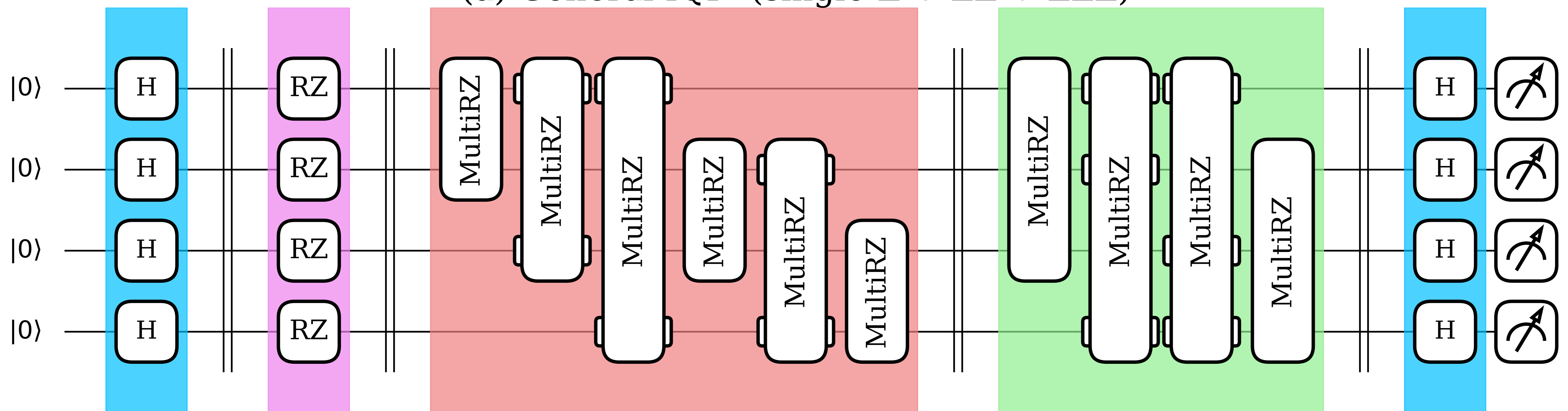
(a) General IQP (single-Z + ZZ + ZZZ)
