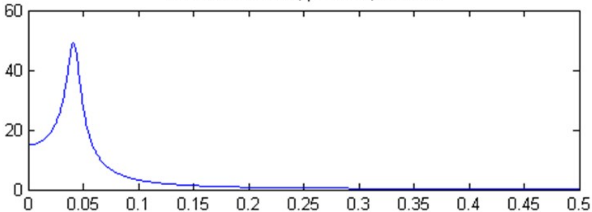
Order 2 AR filter, \rho = 0.96 , \theta = \pi/12
