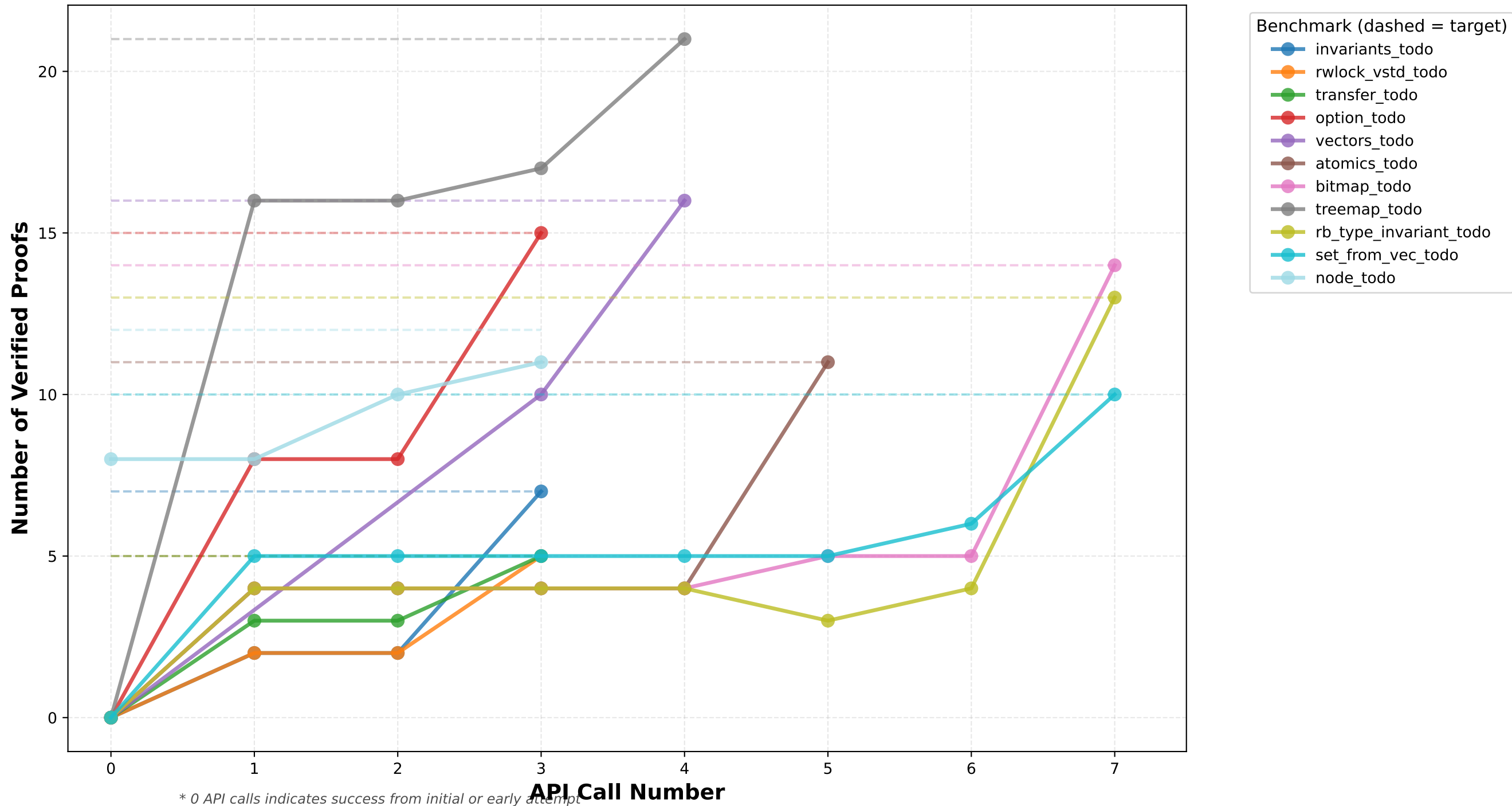
LLM API Call Progression: Verified Proofs Over Time (Per Benchmark)
