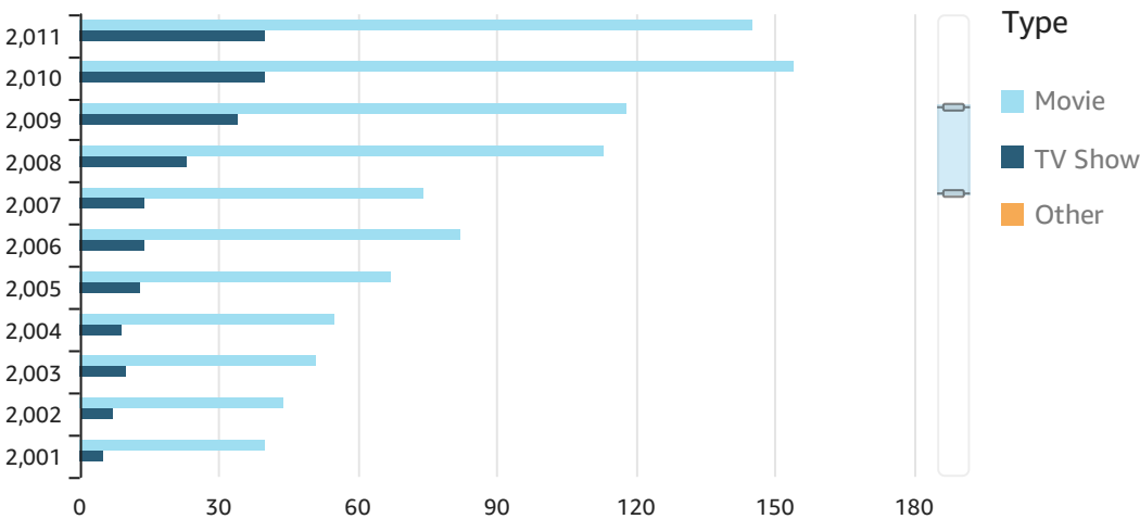
# of Titles Added by Date
