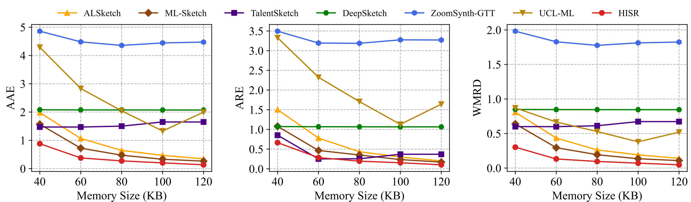
(a) AAE
